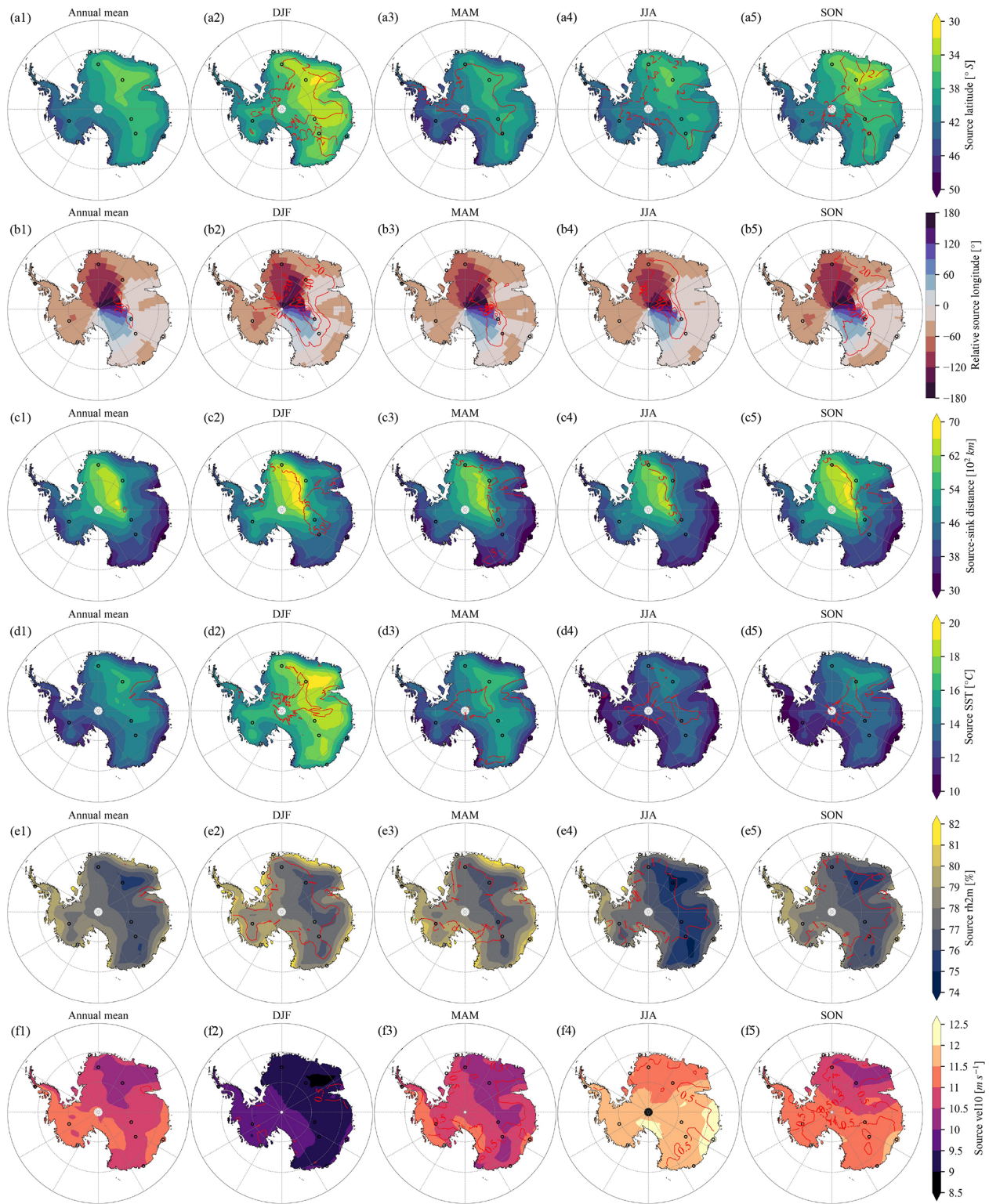
Figure B5. Mass-weighted mean open-ocean evaporative (a) source latitude, (b) relative source longitude, (c) source–sink distance, (d) source SST, (e) source rh_{2m} , and (f) source vel_{10} of the annual mean (the first column) and seasonal mean (the second to fifth columns) precipitation. Red lines show contours of 1 standard deviation. DJF refers to December–January–February, MAM to March–April–May, JJA to June–July–August, and SON to September–October–November.
