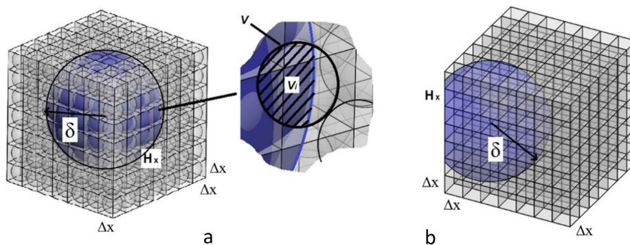
Fig. 3 Numerical spatial integration issues: (a) truncated PD point volumes, requiring volume correction V_i = v_{c_i}V and (b) not full PD horizon at the boundaries, requiring PD bonds stiffness corrections
