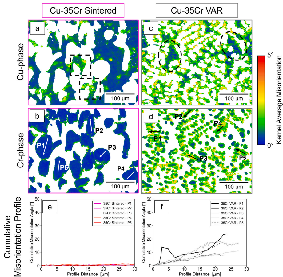
Fig. 5. a-d) Kernel Average Misorientation (KAM) map of the Cu-phase and Cr-phase for the Cu–35Cr SSS and VAR composite. e-f) Cumulative misorientation profiles in the Cr phase measured along the arrows drawn in b) and d).
