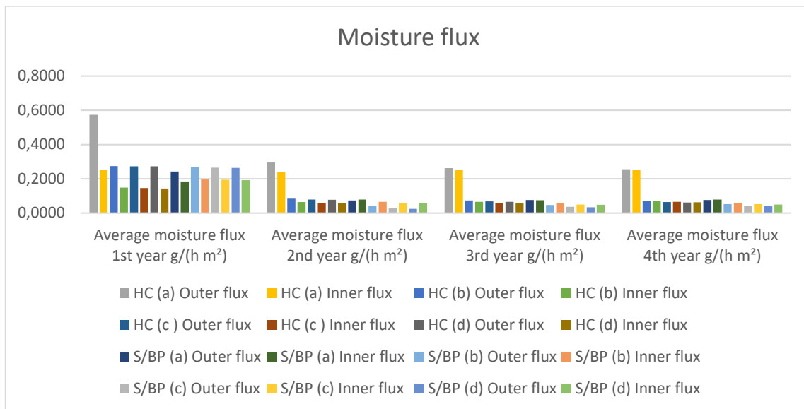
Figure 9: Annual mean inner and outer moisture flux throughout insulation assemblies with S/BP or HC under Nancy's climate
