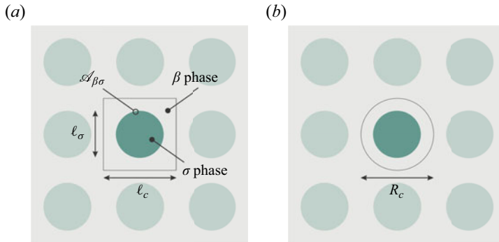
Figure 2. Sketch of a (a) periodic and (b) non-periodic (Chang's) unit cell corresponding to a representation of the porous medium geometry as a square pattern of parallel cylinders of circular cross-section.
