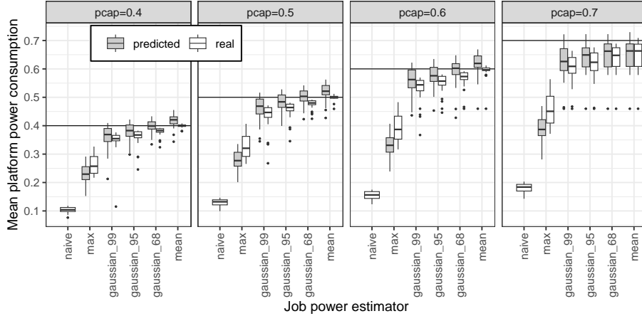
Figure 4: Distribution of the platform power consumption during the powercap-constrained 3-hour time window. The power cap is the horizontal black line. All power values ( y axis, facet powercap \text{pcap} ) are expressed as a proportion of the maximum dynamic power range. Here and in the remaining plots we use standard boxplots, with boxes spanning between the first and the third quartiles, and whiskers reaching the furthers outliers within 1.5 of the interquartile range.
