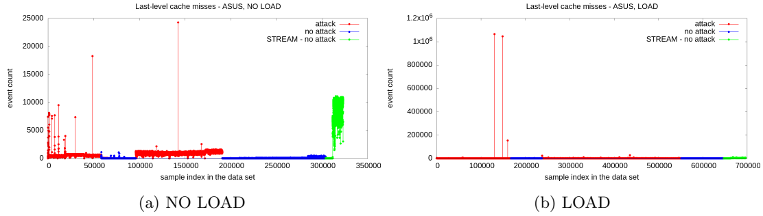
Figure 4: Last-level (L3) cache misses on ASUS machine
