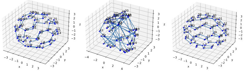
Figure 1: Left: the Buckminsterfullerene molecule with a spiral order on the vertices. Center: wrong realizations obtained for |\delta| = 0.5N . Right: the realization for |\delta| = N yields a perfect reconstruction (rotated).
