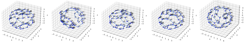
Figure 2: Slightly wrong realizations for |\delta| \in [0.995N, 0.999N] .
