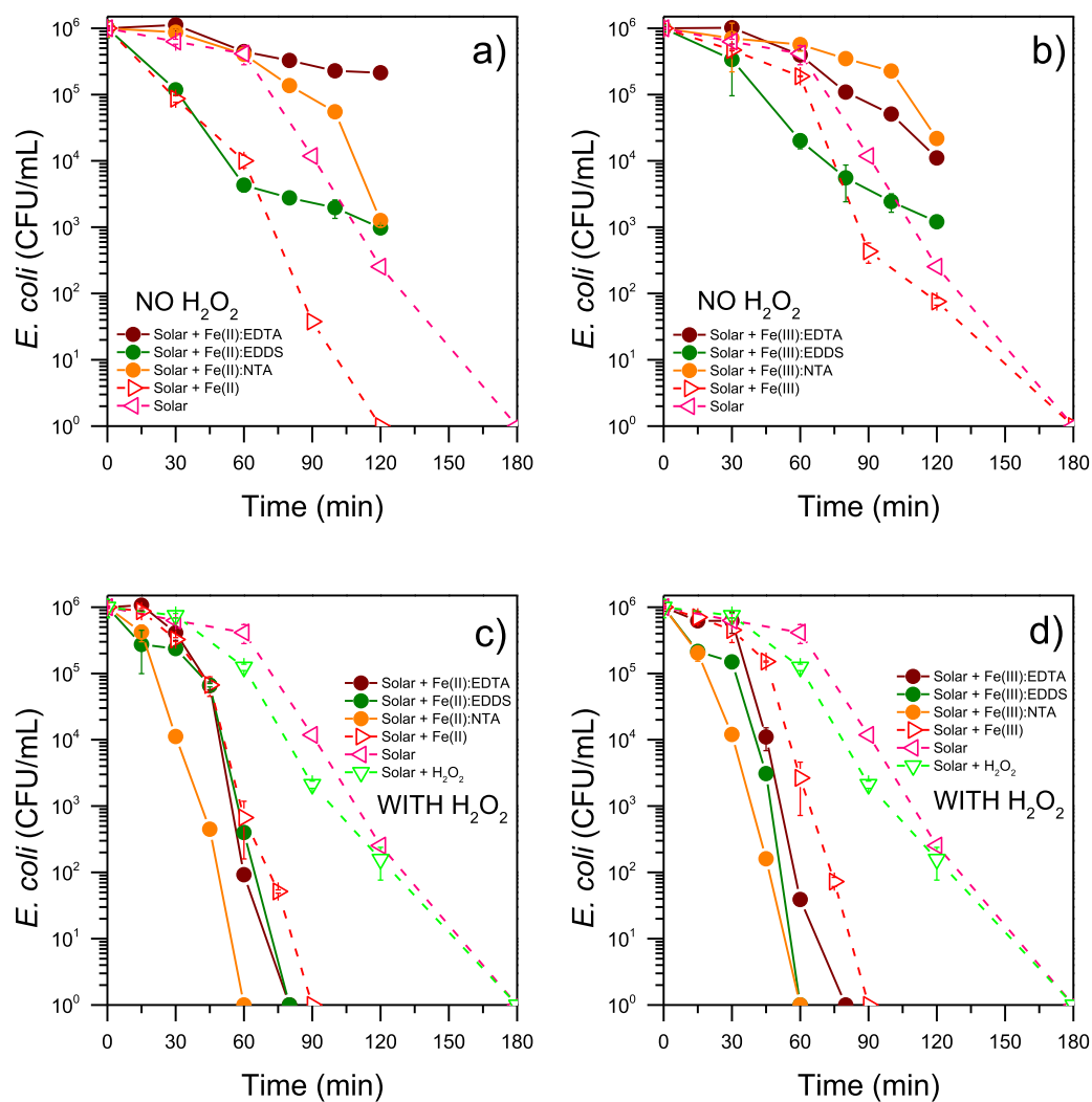
Fig. 6. Bacterial inactivation with iron and iron-synthetic acid complexes (molar ratio 1:2) for EDTA, EDDS, and NTA. A) Solar/ Fe^{2+} -ligand; B) Solar/ Fe^{3+} -ligand; C) Solar/ Fe^{2+} -ligand/ H_2O_2 ; D) Solar/ Fe^{3+} -ligand/ H_2O_2 . The initial conditions were [Fe^{2+,3+}] = 1 \text{ mg/L} , [H_2O_2] = 10 \text{ mg/L} , and 900 \text{ W/m}^2 .
