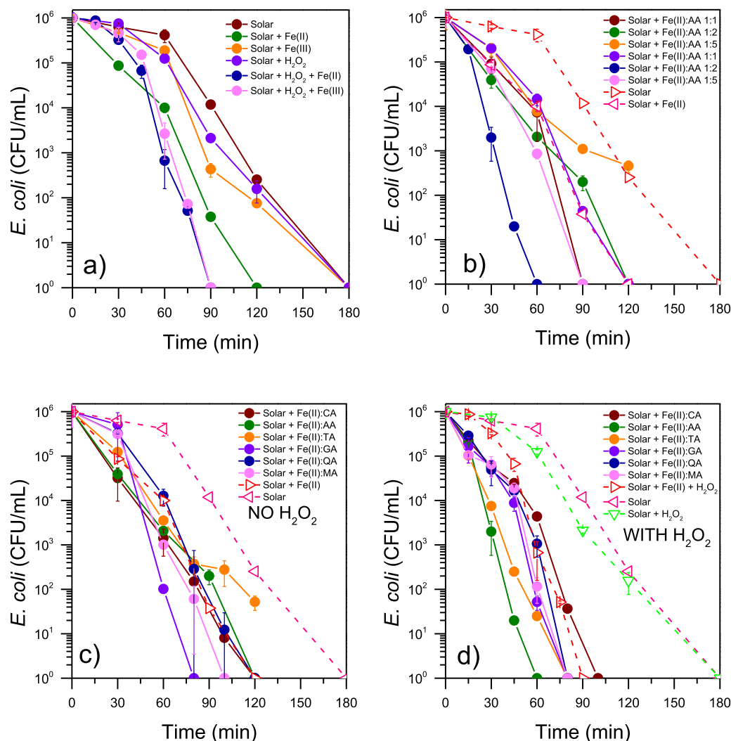
Fig. 5. a) Standard experiments for bacterial inactivation (solar light only, solar + H 2 O 2 , Solar + Fe 2+ , Solar + Fe 3+ , Solar + H 2 O 2 + Fe 2+ , and solar + H 2 O 2 + Fe 3+ ). The initial conditions were [Fe 2+,3+ ] = 1 mg/L, [H 2 O 2 ] = 10 mg/L, and 900 W/m 2 . b) Bacterial inactivation with iron(II)–ascorbic acid complexes at three different molar ratios (1:1, 1:2, and 1:5). Initial conditions: [Fe 2+ ] = 1 mg/L; [H 2 O 2 ] = 10 mg/L; 900 W/m 2 . Figures c) and d) represent bacterial inactivation with iron(II, III)-ligand complexes (molar ratio 1:2), where the ligands were citric, tartaric, ascorbic, malic, glutamic, and quinic acids. c) Solar + Fe + ligand; d) Solar + Fe + ligand + H 2 O 2 . Initial conditions: [Fe 2+ , Fe 3+ ] = 1 mg/L; [H 2 O 2 ] = 10 mg/L; 900 W/m 2 .
