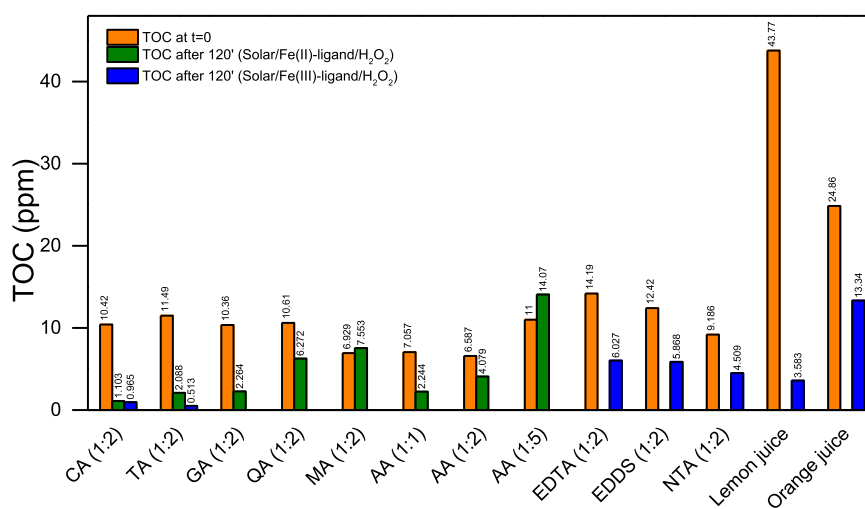
Fig. 7. Initial and final TOC during bacterial inactivation experiments with either Fe^{2+} or Fe^{3+} in the presence of a ligand and H_2O_2 .
