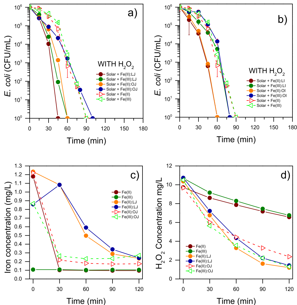
Fig. 8. a) Bacterial inactivation by the photo-Fenton process using lemon and orange juices (LJ and OJ, respectively). b) Bacterial inactivation by the photo-Fenton process with lemon and orange infusions. In both cases, the initial conditions were [Fe^{2+}, Fe^{3+}] = 1 mg/L, [H_2O_2] = 10 mg/L, and 900 W/m 2 , while fruit juices and infusions were dosed, as mentioned in Table 1. Evolution of c) total dissolved iron, and d) H_2O_2 total dissolved iron concentrations in the photo-Fenton process for bacterial inactivation with iron-synthetic acid complexes (EDTA, EDDS, and NTA).
