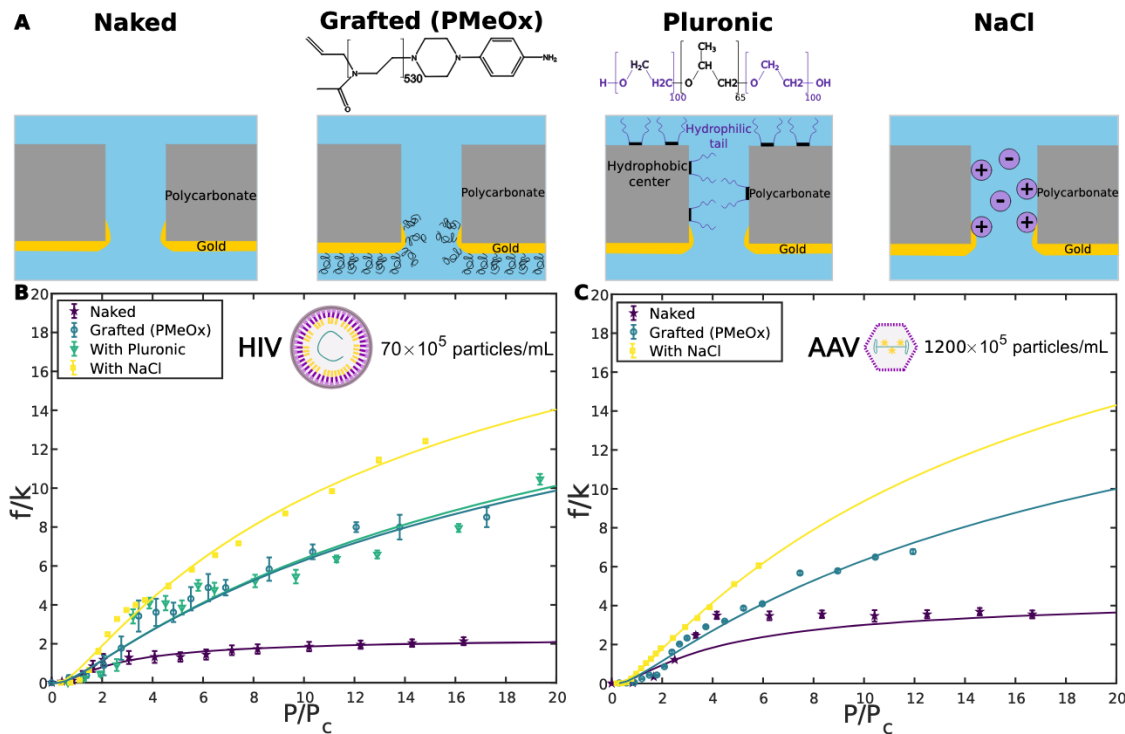
Fig. 4 | Chemical Environment Modifications. A Schematic representation of the nanopore environment. From left to right: naked nanopore; nanopore grafted with synthetic polymers (PMeO x , polymerization degree of 530) on the gold side; nanopore passivated with Pluronic; nanopore in the presence of 150 mM NaCl. B HIV translocation for different nanopore environments. Evolution of normalized translocation frequency as a function of normalized pressure for HIV particles for different nanopore environments: naked, grafted (PMeO x ), passivated (Pluronic), with NaCl (150 mM). The translocation frequency was higher for grafted and passivated membranes and even higher with salt compared to naked membranes. The
