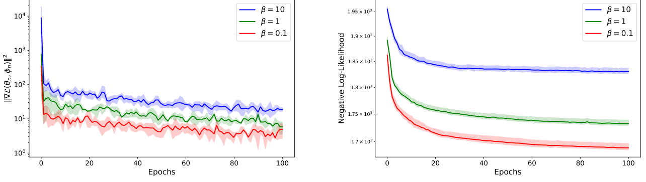
Figure 6: Squared norm of gradients (on the left) and Negative Log-Likelihood (on the right) for \beta -VAE trained on CIFAR-100 dataset using Adam. Bold lines represent the mean over 5 independent runs.
