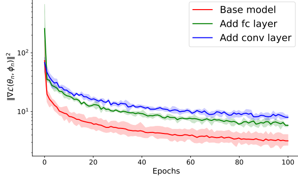
Figure 4: \|\nabla\mathcal{L}(\theta_n, \phi_n)\|^2 in VAE trained with Adam for the baseline model, a model with an additional fully connected layer, and a model with an additional convolutional layer. Bold lines represent the mean over 5 independent runs. Figures are plotted on a logarithmic scale for better visualization.
