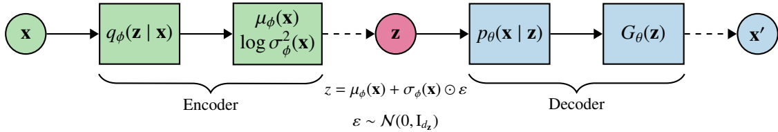
Figure 3: Illustration of the Architecture of a VAE with the Multivariate Gaussian.
