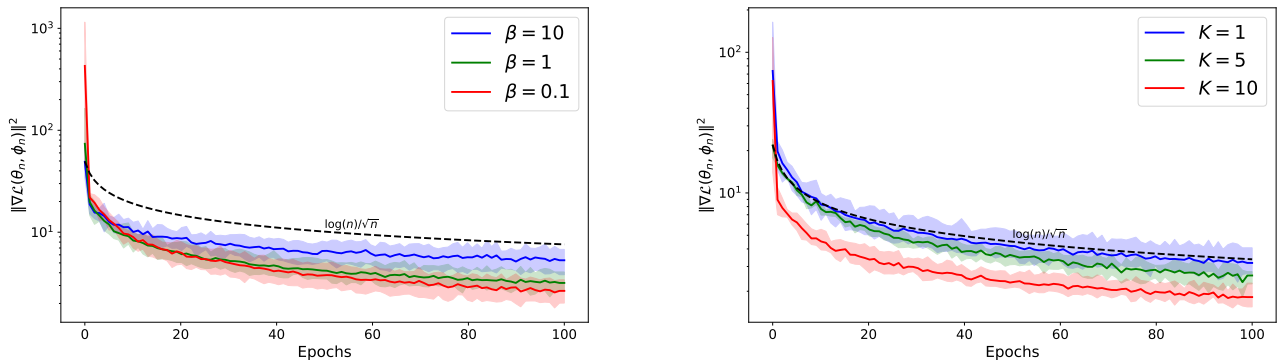
Figure 2: \|\nabla \mathcal{L}(\theta_n, \phi_n)\|^2 in \beta -VAE (on the left) and IWAE (on the right) trained with Adam. Bold lines represent the mean over 5 independent runs. The dashed curves correspond to the expected convergence rate O(\log n / \sqrt{n}) .
