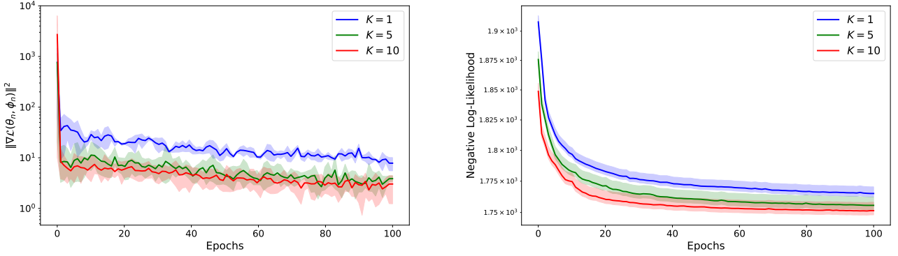
Figure 7: Squared norm of gradients (on the left) and Negative Log-Likelihood (on the right) for IWAE trained on CIFAR-100 dataset using Adam. Bold lines represent the mean over 5 independent runs.
