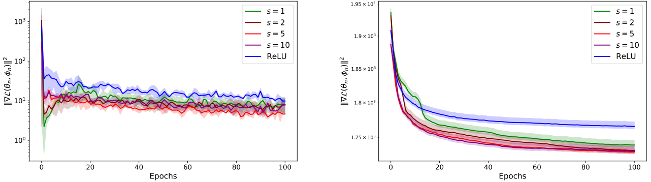
Figure 5: Squared norm of gradients and Negative ELBO on the test set of the CelebA for VAE trained with Adam and generalized soft-clipping activation function. Bold lines represent the mean over 5 independent runs.
