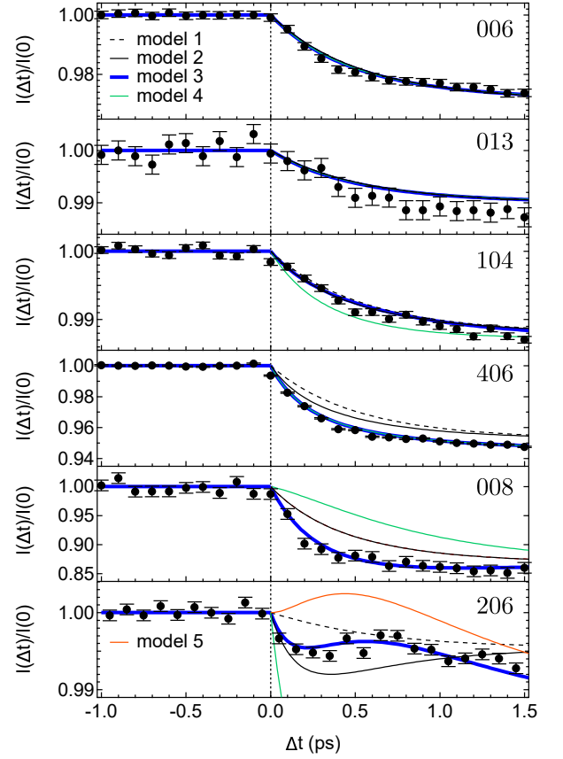
FIG. 3. (Color online) Symbols : time-resolved diffraction measurements of the 006, 013, 104, 406, 008, 206 Bragg reflections of ferromagnetic \alpha -MnAs at T=282 \text{ K} , pump fluence of 1.5 \text{ mJ}\cdot\text{cm}^{-2} . Lines : model calculations based on Eqs. (2-7). Model 1: all time constants set to 550 fs. Model 2: \tau_{11}^{\text{As}}=160 \text{ fs} , the others are set to 550 fs. Model 3: \tau_{11}^{\text{Mn}}=700 \text{ fs} , \tau_{11}^{\text{As}}=160 \text{ fs} , \tau_{22}^{\text{Mn}}=\tau_{33}^{\text{Mn}}=400 \text{ fs} , \tau_{22}^{\text{As}}=\tau_{33}^{\text{As}}=700 \text{ fs} . Model 4: \tau_{11}^{\text{Mn}}=700 \text{ fs} , \tau_{11}^{\text{As}}=160 \text{ fs} , \tau_{22}^{\text{Mn}}=\tau_{33}^{\text{Mn}}=700 \text{ fs} , \tau_{22}^{\text{As}}=\tau_{33}^{\text{As}}=400 \text{ fs} . Model 5 (for 206 reflection only): variation on model 3, with \tau_{11}^{\text{Mn}}=160 \text{ fs} . Model 1 to 4 are represented for each reflection (they superimpose for 006 and 013).
