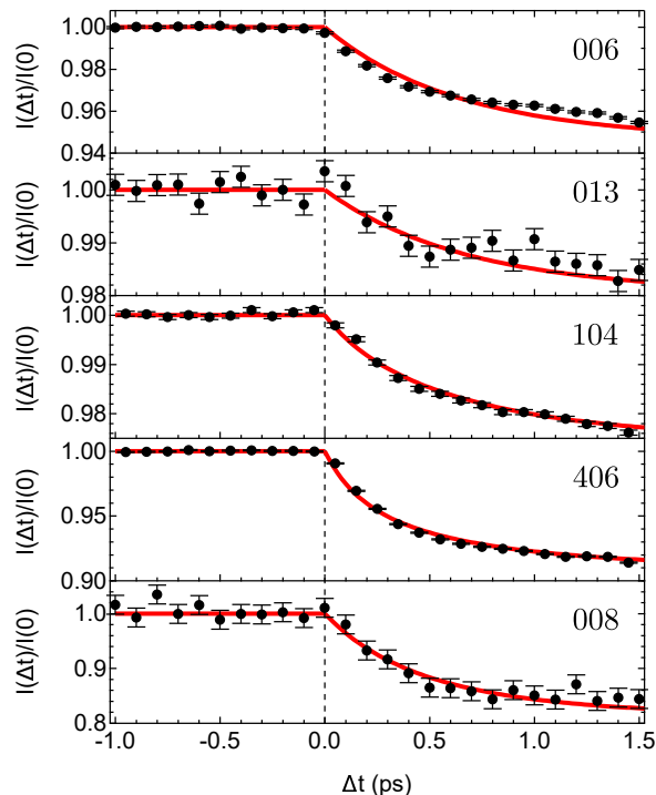
FIG. 4. (Color online) Symbols: time-resolved diffraction measurements of the 006, 013, 104, 406, 008 Bragg reflections of paramagnetic MnAs at T=404 K, pump fluence of 1.5 \text{ mJ.cm}^{-2} . Lines: model calculations with \tau_{11}^{\text{As}}=160 fs, the others \tau_{ii}^X are set at 700 fs.
