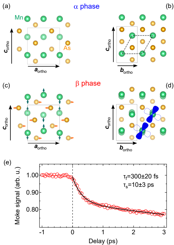
FIG. 1. (Color online) Crystallographic structure in the \alpha phase (a-b) and \beta phase (c-d) of MnAs. Arrows in (c) indicate the direction and sense of the atomic displacements involved in the hexagonal to orthorhombic transition. In (d) the Mn d_{x^2-y^2} orbitals in the hexagonal planes are depicted in blue. The crystal structures were drawn with VESTA [18]. (e) Ultrafast demagnetization curve of MnAs/GaAs(001) at T=278 K, pump fluence 1 \text{ mJ.cm}^{-2} . Symbol: experimental points, line: fit to equation (1).
