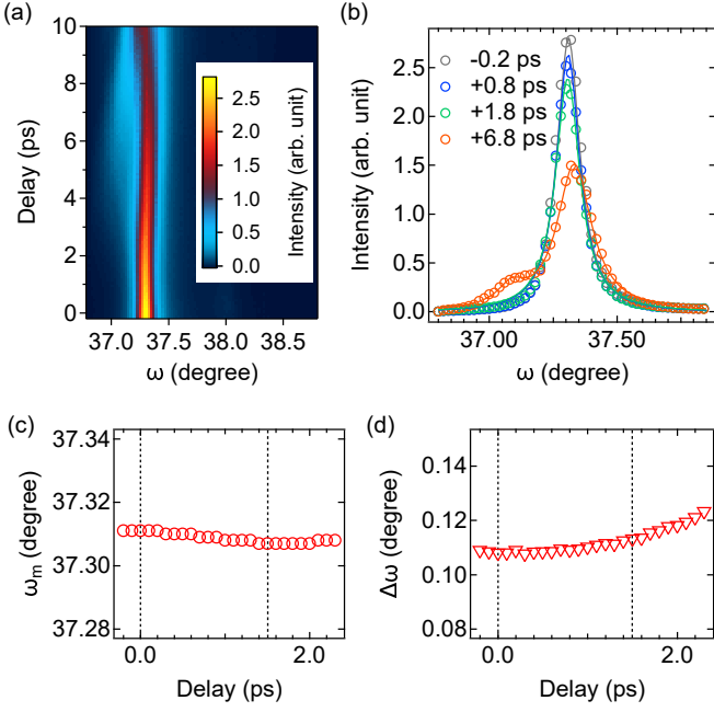
FIG. 2. (Color online) Time-resolved diffraction measurements of the 006 Bragg reflection. (a) Map of the diffracted intensity as a function of the incidence angle \omega and of the delay \Delta t . (b) Profiles at selected delays. Circles: data, lines: fits using lorentzian profiles. Fitted peak position (c) and peak width (d) as a function of \Delta t . Pump fluence 5 \text{ mJ}\cdot\text{cm}^{-2} .
