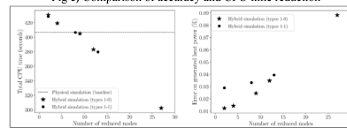
Fig e) Comparison of accuracy and CPU time reduction
