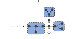
Fig b) Graph formulation of the original DHN
