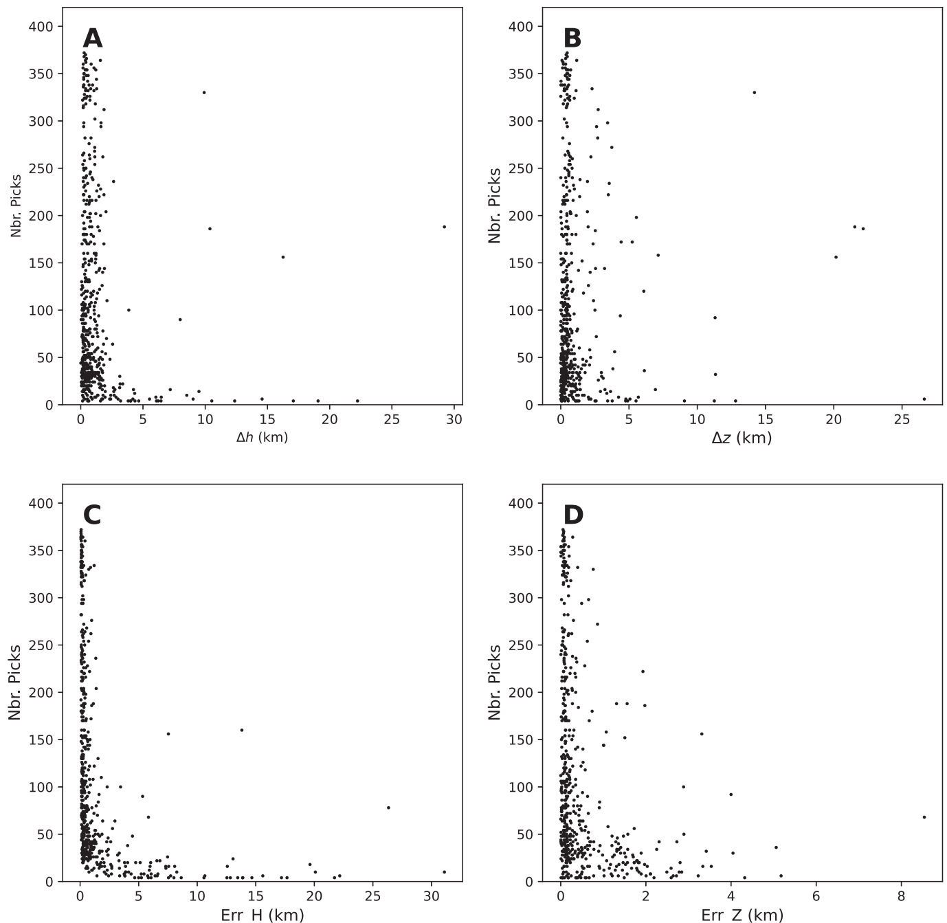
Fig. 13. Influence of the 3D velocity model on hypocenter locations. Horizontal (A) and vertical (B) distance between 1D and 3D hypocenter locations versus number of picks. Horizontal (C) and vertical (D) statistical errors in the 3D model versus number of picks.
