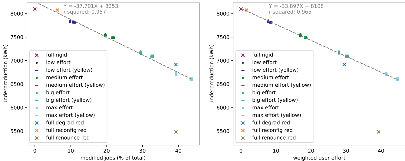
(a) “effort” in number of jobs modified (Table III, 3rd column) (b) “effort” expressed with weighted effort (Table IV, last column)
