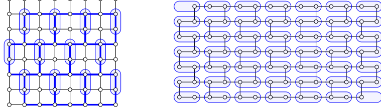
■ Figure 2 Proof by picture of the two items of Lemma 6: \Gamma_8 admits a W_4 induced minor (left) and W_7 admits a \Gamma_7 induced minor (right). The shaded boxes represent the contractions to perform. The vertices not incident to a blue edge (left) should be deleted.
