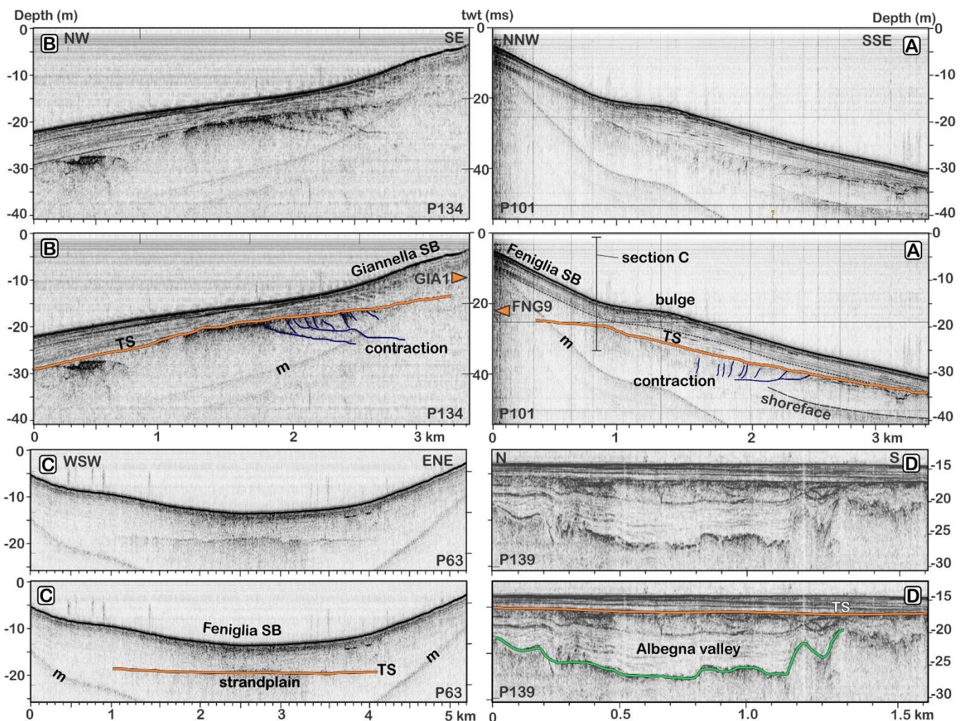
Figure 7. Raw and interpreted 3.5 kHz offshore acoustic profiles across the Feniglia (A) and Giannella (B) sand barrier shorefaces (location: Fig. 2A). TS: transgression surface. m: first multiple. Orange triangle point to the depth of the depth of the transgression surface in cores onshore.
