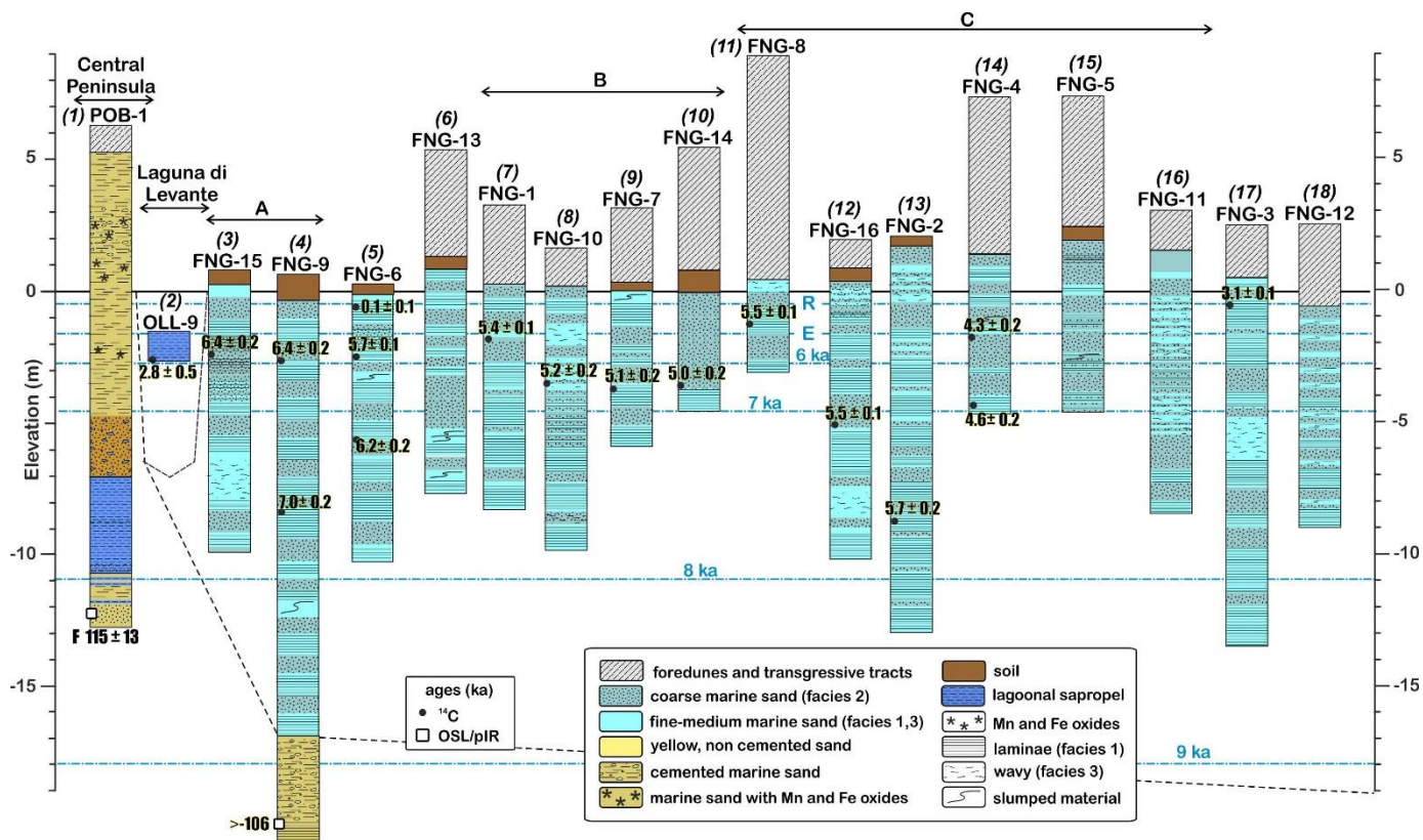
Figure 5. Distribution of sediment facies and ages along a core transect from the Central Peninsula to the Feniglia sand barrier. Italic numbers in brackets next to core names: core locations of Figs. 4 and 5. Black dashed line: sequence boundary. A, B, and C: beach ridgelines (Fig. 2C). Black long-dashed line: sequence boundary. Black, short-dashed line: base of lagoon layers. Blue dashed lines: sea level at successive 1 ka time step according to the model curve of Roy and Peltier (2018). Roman (R) and Etruscan (E) levels from Leoni and Dai Pra (1997).
