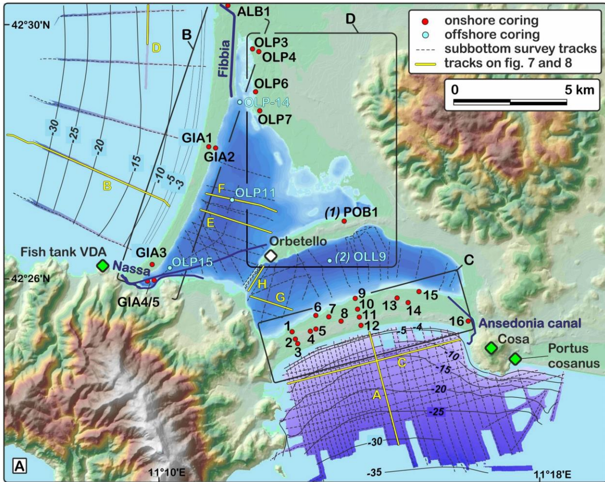
Figure 2. Coring and sub-bottom profile locations. (A) general map of Orbetello. VDA: Fish tank of Villa Domitius Ahenobarbus. Land topography: 10 m-resolution DTM (CC-BY, Regione Toscana). Offshore bathymetry: 10 m-resolution DEM (Brocard and Conforti, 2023), with contour lines every 5 m below -5 m, and every 1 m above -5 m. Lagoon bathymetry digitized from Cappiotti et al. (2006). B: topography of the Giannella sand barrier, C: topography of the Feniglia sand barrier. D: topography of the central peninsula and of the Patanella area. Land topography on B, C, and D: 2 m-resolution LiDAR DTM (Ministero della Transizione Ecologica CC BY 3.0). Ancient settlement locations from (Dolci, 2014; Negroni Catacchio et al., 2019). Bracketed numbers in italic: core order as displayed on the transects of Figs. 4 and 5.
