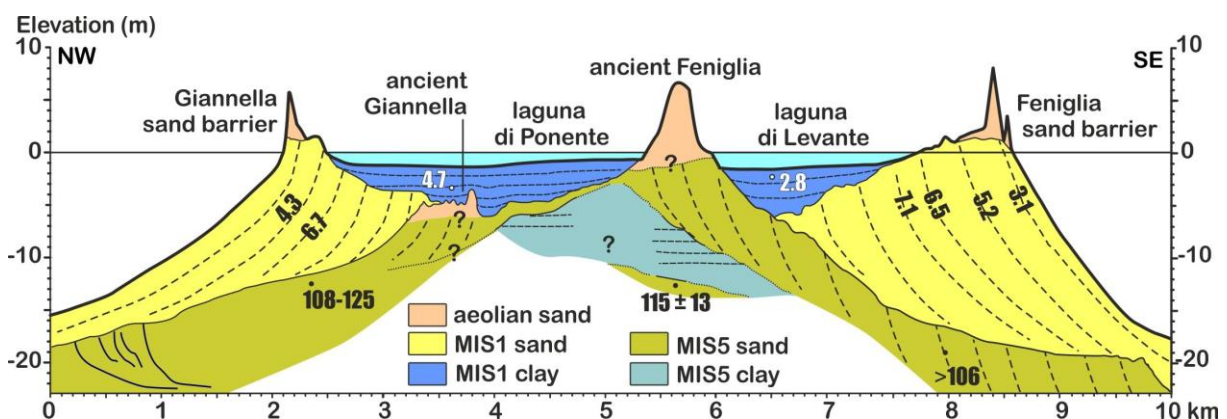
Figure 10. Synthetic section across the peninsula of Orbetello, showing the main elements of its sedimentary architecture. Numbers in bold indicate accretion age (in ka) based on ^{14}\text{C} , luminescence, and U/Th ages.
