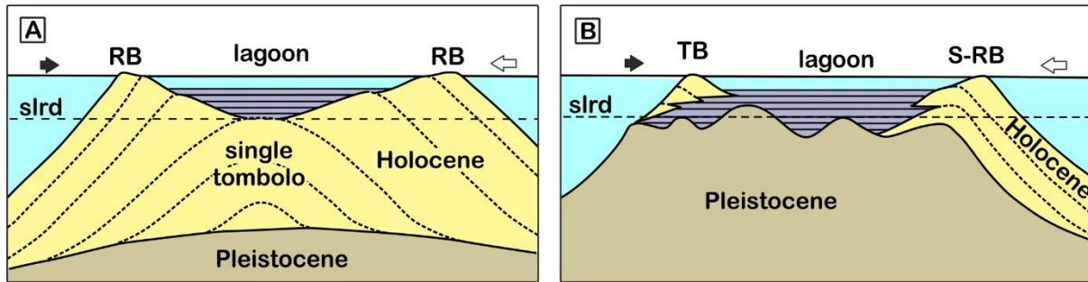
Figure 12. Conceptual model showing the formation of a double tombolo composed of flooded regressive barriers (A), and transgressive, stationary to regressive barriers (B). slrd: sea level rise deceleration. RB: regressive barrier, TB: transgressive barrier, S-RB: stationary to regressive barrier. White/black arrows: dominant/minor longshore sediment flux.
