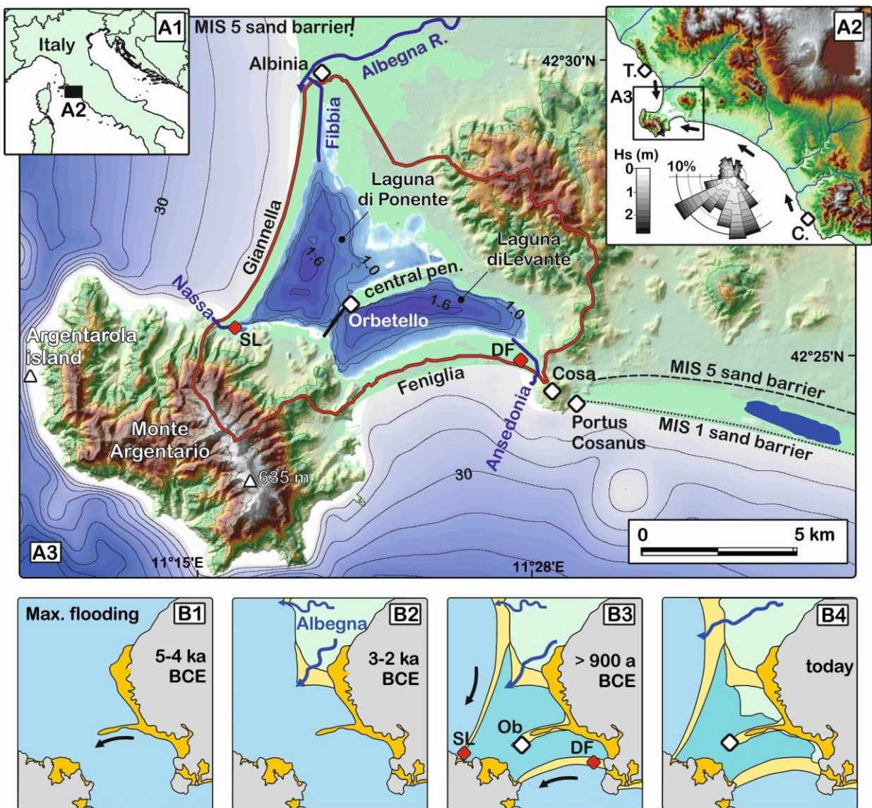
Figure 1. Study area in Italy (A1), and Tuscany (A2), showing longshore drift directions (arrows), and a rose diagram of the yearly distribution of incoming waves (in % of time) as a function of significant wave height ( H_s ). Data from MEDATLAS, tile 42N11E (MEDAR_Group, 2002). C and T: towns of Civitavecchia and Talamone. A3: topography and main features. Red line: watershed of the lagoon of Orbetello. Blue lines: canals connecting the lagoon to the sea and rivers. White diamonds: Etruscan-Roman settlements (Ob: Orbetello). Red diamonds: Late Bronze Age settlements (DF: Duna Feniglia; SL: Santa Liberata). Contour line values in meter. Lagoon bathymetry digitized from Cappiotti et al. (2006). Onshore topography: 10 m-resolution DTM (CC-BY, Regione Toscana). For color colour scale see Fig. 2. Bathymetry: GMRT grid version 11.4, CC BY (Ryan et al., 2009) extracted using GeoMapApp ( www.geomapp.org ) CC-BY. Panels B1-B4: paleogeographic evolution, combining key elements of the models by Coltorti and Ravani (2017) and D'Orefice et al. (2022). B1: maximum Holocene flooding. B2: growth of the Albegna River delta in open marine environment. B3: growth of the Holocene sand barriers before the Late Bronze Age. B4: final closure of the lagoon. (For interpretation of the references to colour in this figure legend, the reader is referred to the web version of this article.)
