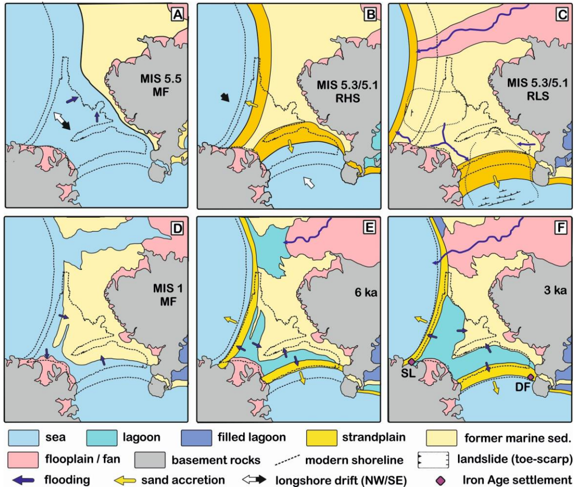
Figure 11. Geographic evolution of the double-tombolo system of Orbetello. A: Last interglacial maximum flooding (MF, MIS5.5, ca. 130–120 ka); B: relative highstand (RHS) during MIS 5.3 to 5.1 stadial substages (ca. 100–80 ka); C: relative lowstand during MIS 5.3 to 5.1; D: Holocene (MIS 1) maximum flooding (MF); E: lagoon formation and expansion (6 ka); F: Late Bronze age (3 ka).
