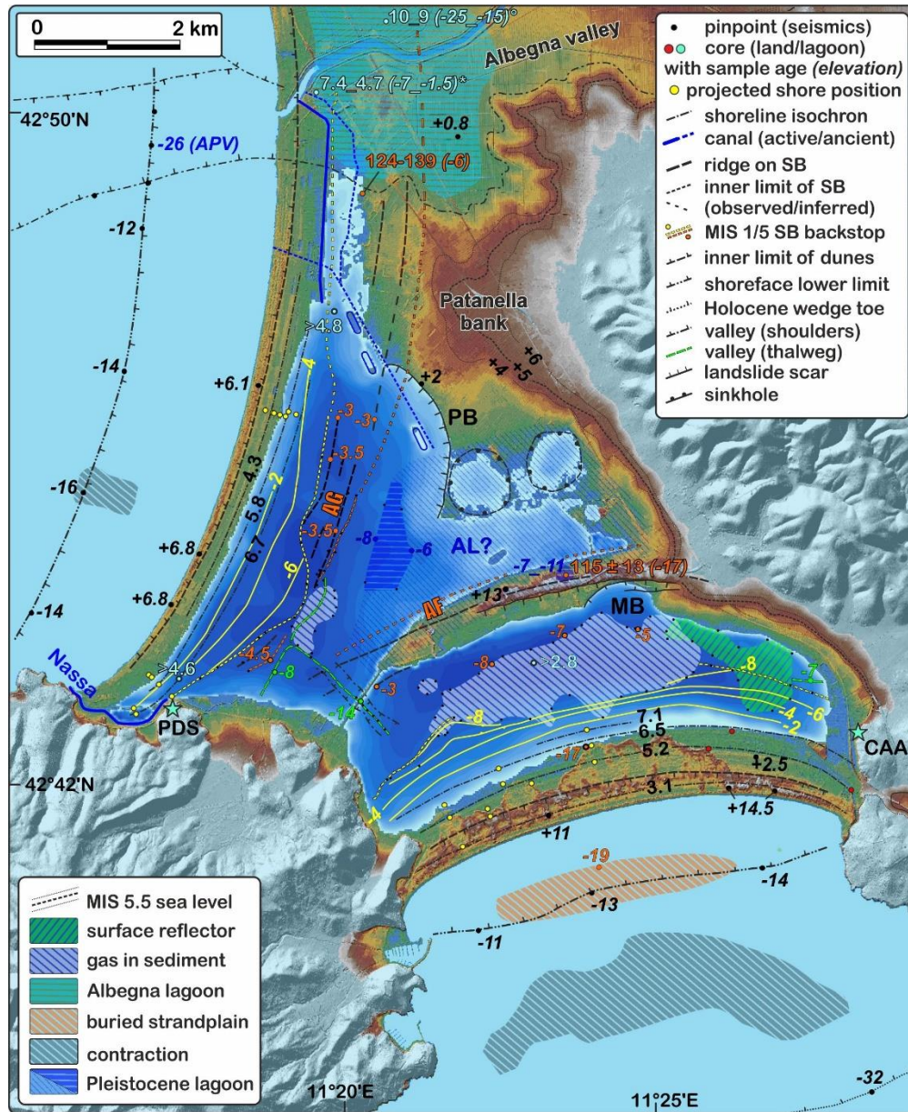
Figure 9. Map of the tombolo of Orbetello showing morphological features emplaced since the last interglacial. Numbers in italic : elevations amsl in meters (black: modern surface; green: MIS 4–2 paleovalley thalwegs, yellow: contour lines on MIS 1 ridge plain surfaces; orange: MIS 5 surfaces; blue: ancient lagoon layers), other numbers: age in ka of samples dated in this study (with elevation in italic ) and of calculated paleoshoreline positions. Earlier published ages from: ° (Mazzini et al. , 1999), * (Chapkanski et al. , 2022). AG: ancient Giannella, AF: ancient Feniglia, AL?: putative ancient lagoon, APV: Albegna paleovalley; CAA: Cosa-Ansedonia aquifer; MB: La Madonnella Bight; PB: Patanella Bight; PDS: Punta degli Stretti cave.
