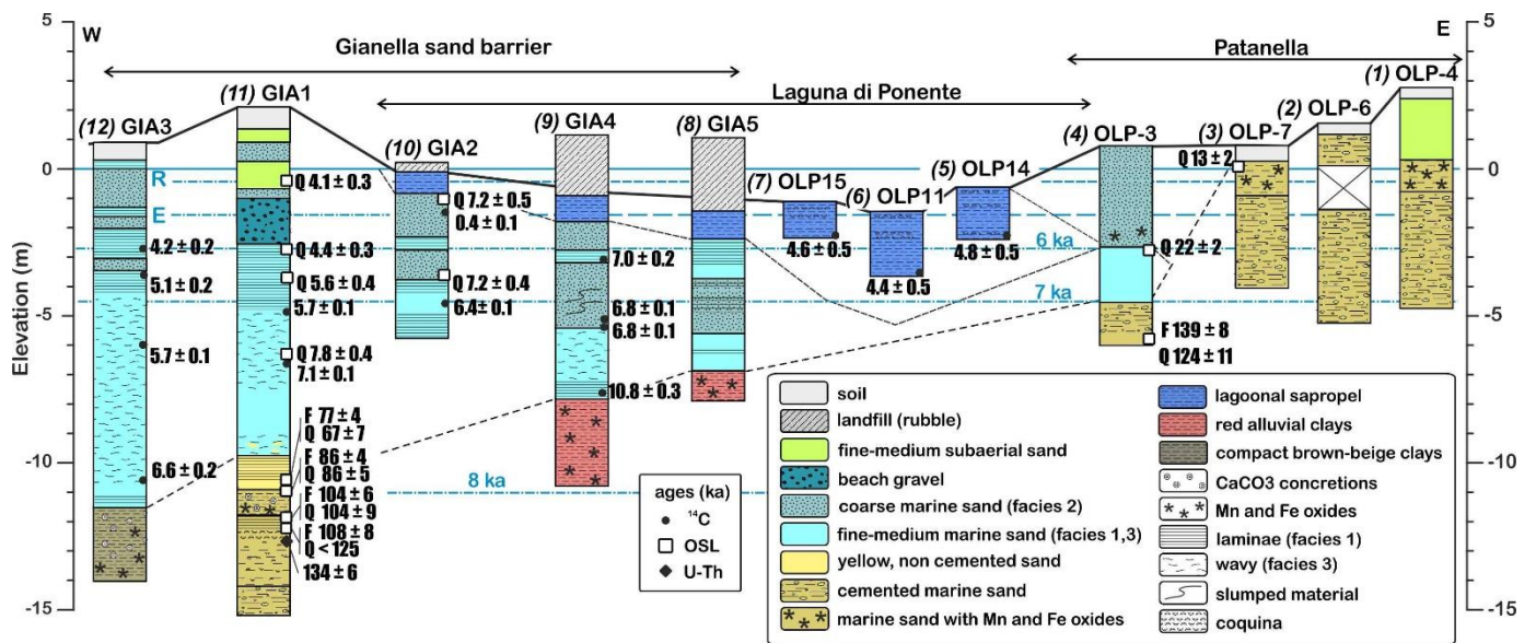
Figure 4. Distribution of sediment facies and ages along a core transect from the Patanella bank to the Giannella sand barrier. Black long-dashed line: sequence boundary. Black, short-dashed line: base of lagoon layers. Blue dashed lines: sea level at successive 1 kyr time step according to the model of Roy and Peltier (2018). Roman (R) and Etruscan (E) levels from Leoni and Dai Pra (1997).
