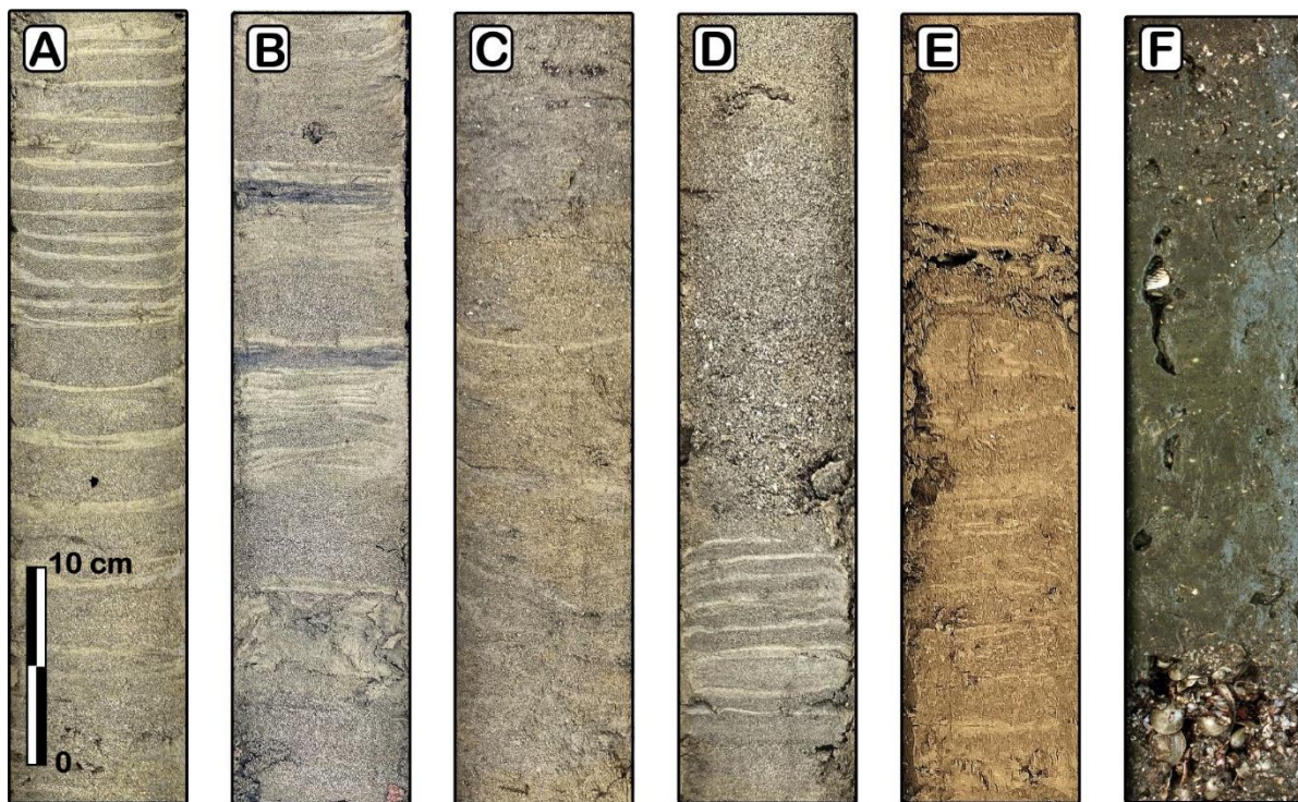
Figure 3. Photographs showing the most commonly cored facies. A: alternation of sand and silty-clayey sand laminae (facies 1, FNG-11, -8.4 m). B: alternation of laminated silty sand and homogenous medium sand (FNG-10, -3.7 m). C: sands of facies 3 (GIA-3, -8.5 m). D: facies 2: coarse, homogenous, fining-upward sand with basal unconformity over laminated alternations of fine sand and silty sand of facies 1 (FNG-9, -10.1 m). E: Pleistocene marine sand, facies similar to facies 1 (FNG-9, -21.2 m). F: Holocene lagoonal, organic rich, shelly sapropel with coquina levels (OLP-15, -1.5 m).
