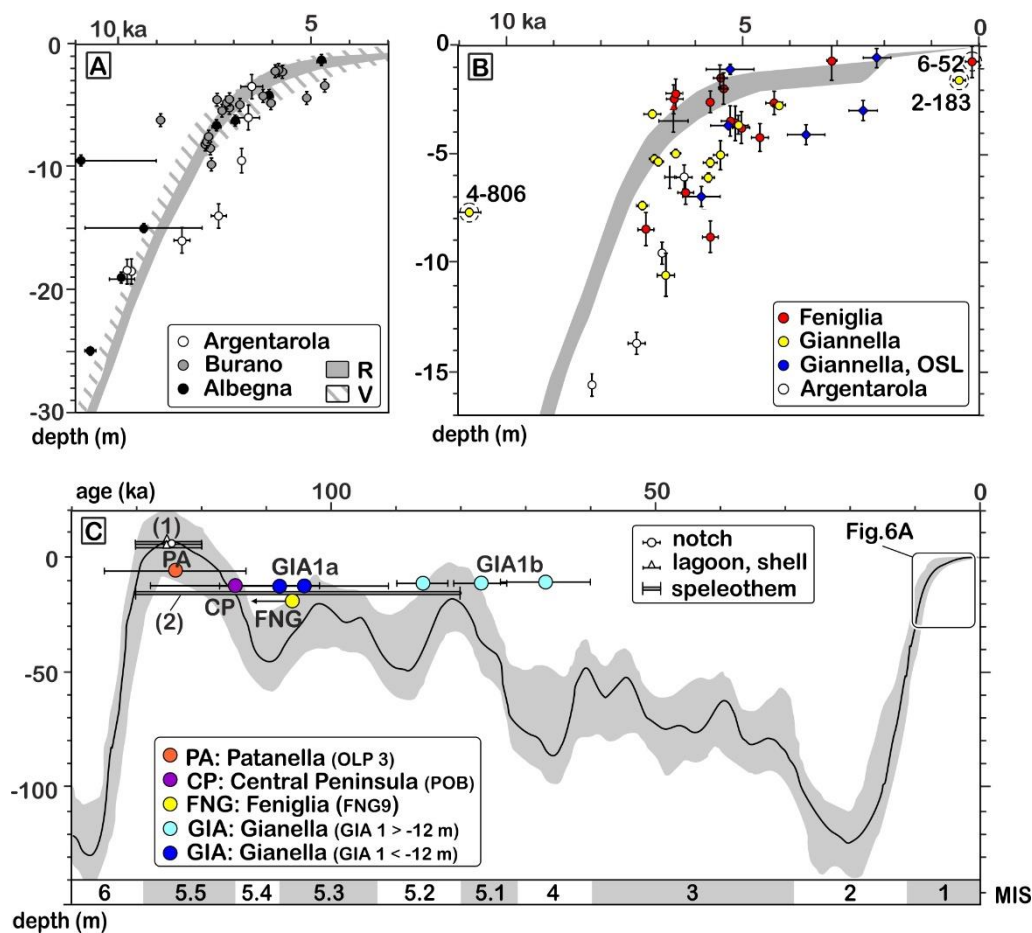
Figure 6. Sea level rise curves compared to ^{14}\text{C} and OSL deposition ages in the sand barriers. A: Albegna estuary, Burano lagoon, and Argentarola cave post-glacial sea level indicators, plotted against the modeled sea level curves for the Northern Latium (R and V, see text for references). Sample numbers refer to outliers mentioned in the text. B: plot of Holocene ^{14}\text{C} (all symbols but blue) and luminescence ages (blue) ages of marine samples vs. depth, relative to the Roy and Peltier (2018) curve, modified over the past 2.5 kyrs to include local archeological constraints from Leoni and Dai Pra (1997). C: Sea level curve of the past 130 ky (Waelbroeck et al., 2002), and last interglacial local sea level indicators: notch and marine/lagoonal fauna (Nisi et al., 2003), interrupted speleothem growth, Argentarola cave (Antonoli et al., 2004), and OSL data (this study). MIS: marine isotopic stages.
