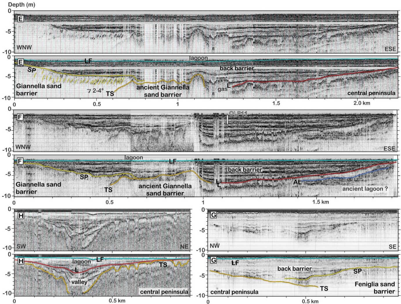
Figure 8. Raw/interpreted 10 kHz acoustic profiles across the lagoon of Orbetello (location: Fig. 2A). Lines: AL: erosion surface of ancient lagoon layers, L: base of modern lagoon layers, LF: lagoon floor, SP: strandplain, TS: transgression surface.
