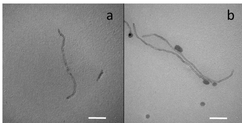
131 132 Figure 1. Transmission electron micrographs of individual Arkema (a) and Nanocyl (b) MWCNT 133 after sonication. Scale 100nm.
