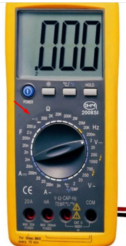
Figure 20 Le mode diode
