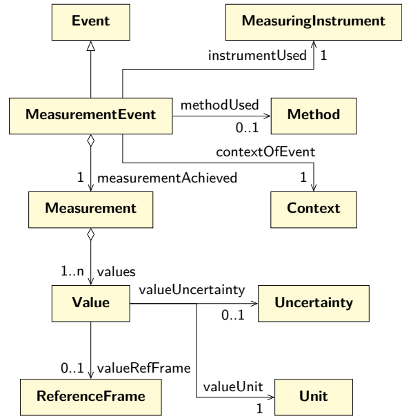
Figure 3: Simplified generic measurement domain model.
