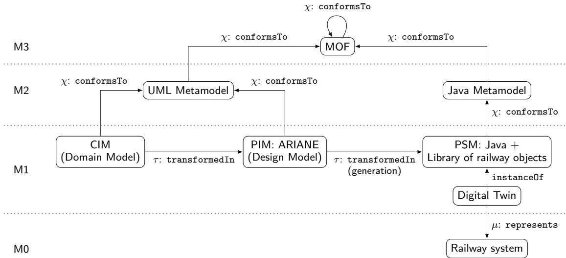
Figure 2: Synoptic megamodel of our framework for producing a DT, applied at SNCF RÉSEAU.
