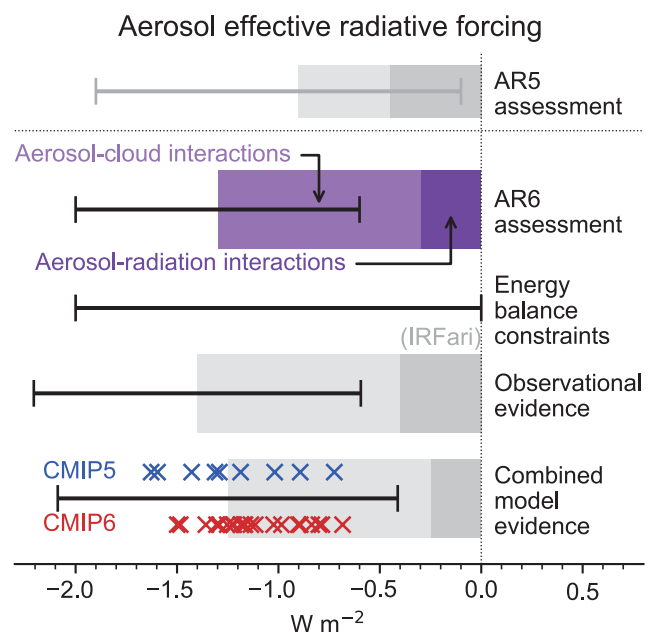
Figure 7.5 | Net aerosol effective radiative forcing (ERF) from different lines of evidence. The headline AR6 assessment of -1.3 [ -2.0 to -0.6 ] W m^{-2} is highlighted in purple for 1750–2014 and compared to the AR5 assessment of -0.9 [ -1.9 to -0.1 ] W m^{-2} for 1750–2011. The evidence comprising the AR6 assessment is shown below this: energy balance constraints [ -2 to 0 W m^{-2} with no best estimate]; observational evidence from satellite retrievals of -1.4 [ -2.2 to -0.6 ] W m^{-2} ; and climate model-based evidence of -1.25 [ -2.1 to -0.4 ] W m^{-2} . Estimates from individual CMIP5 (Zelinka et al., 2014) and CMIP6 (Smith et al., 2020b and Table 7.6) models are depicted by blue and red crosses respectively. For each line of evidence the assessed best-estimate contributions from ERF ari and ERF aci are shown with darker and paler shading respectively. The observational assessment for ERF ari is taken from the IRF ari . Uncertainty ranges are represented by black bars for the total aerosol ERF and depict very likely ranges. Further details on data sources and processing are available in the chapter data table (Table 7.SM.14).
