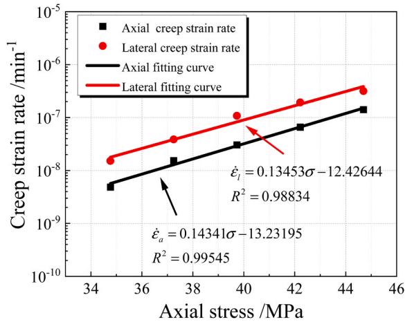
Fig. 11. Variations of axial and lateral creep strain rates against axial stress.
