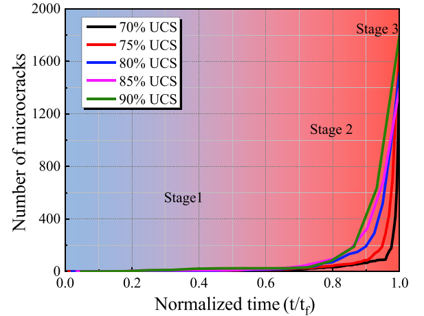
Fig. 13. Variation of the number of microcracks with normalized time for uniaxial creep simulations performed at different stress levels.
