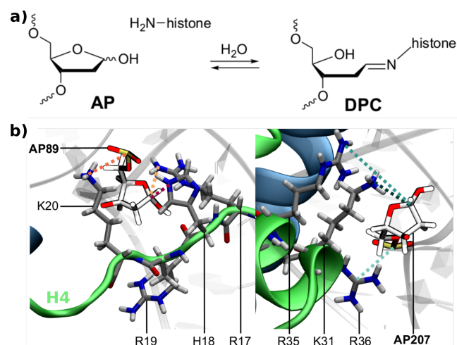
Figure 3. a) Schematic representation of an abasic site (AP) isolated (left) or involved in a DPC (right). b) Mapping of the interactions between histone H4 basic residues and clustered abasic sites (positions 89 and 207) in the nucleosome from MD simulations. Adapted from (Bignon et al. 2021).
