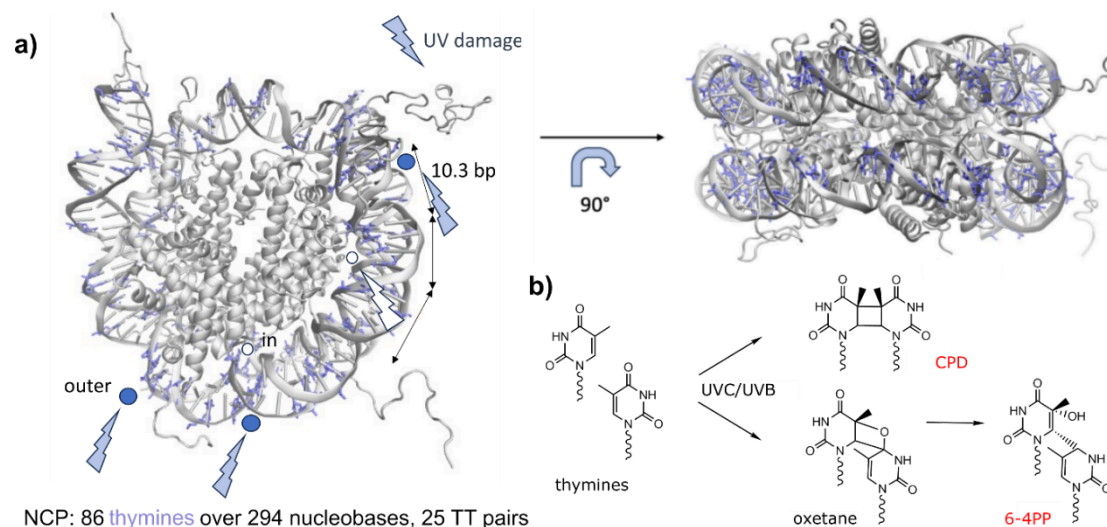
Figure 4. a) Thymine positions over an \alpha -satellite nucleosome (front and top views). Formation yields obey a 10.3 base pair periodicity, with more propensity when they face outward (outer) the histone core than inwards (in). b) Structure of the two main DNA photolesions: cyclobutane pyrimidine dimers (CPD) and pyrimidine 6-4 pyrimidone (6-4PP).
