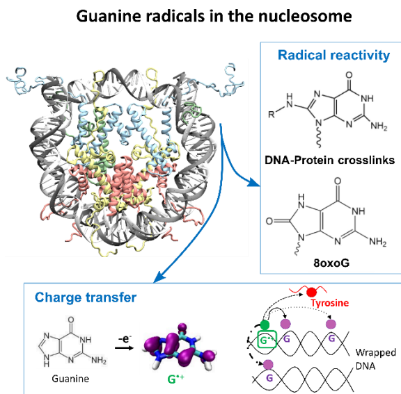
Figure 2. Guanine radical cation evolution in the nucleosome, leading to the formation of crosslinks, 8-oxoguanine, or charge transfer within DNA or towards tyrosines.
