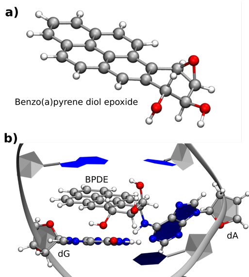
Figure 5. a) 3D structure of the benzo(a)pyrene diol epoxide (BPDE) compound. b) Crystal structure of a BPDE-dA adduct in B-DNA, with a facing dG mismatch (Schwartz et al. 1997).
