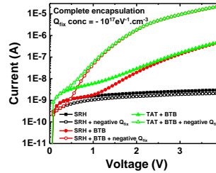
Fig. 15: Impact of Q_{\text{fix}} on the I_{\text{dark}} vs V including different transport mechanisms
