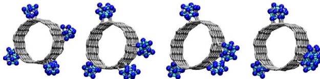
Figure 3: Panels from left to right show the dynamical evolution of the four Co nanoclusters on the (10,10) CNT during our canonical NVT simulation resulting in the formation of larger Co cluster which remains stable on the time scale of our FPMD. The color code is the same used in former figures.
