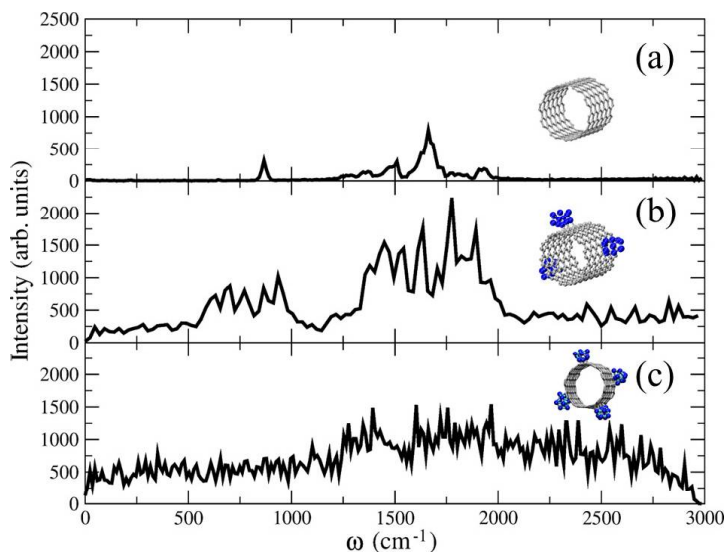
Figure 1: Simulated IR absorption spectra for (a) the (10,10) carbon nanotube, (b) the same nanotube decorated with three Co nanoclusters, and (c) decorated with four Co nanoclusters. The inset figures are a graphic reminder of the system to which each spectrum refers and the color code is gray for C and blue for Co.
