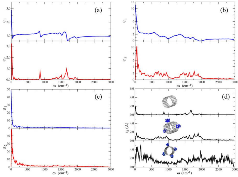
Figure 5: Real (blue lines) and imaginary (red) part of the complex dielectric function for the bare (10,10) CNT (a) the same CNT decorated with three (b) and four (c) Co nanoclusters. Panel (d) shows the three dielectric loss tangent curves for these three systems with the same labeling and the inset figures are a reminder of the system to which they refer.
