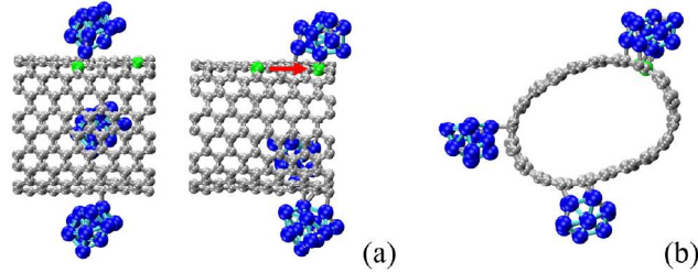
Figure 2: Evolution of the (10,10) CNT decorated with three Co nanoclusters. (a) displacement of the Co nanoclusters during the NVT dynamics. The C atoms highlighted in green show the initial position of one of the three clusters (left) where a C–Co chemical bond exists and (right) displaced position assumed by this same Co nanocluster after 8.7 ps along the direction indicated by the arrow, where a new C–Co chemical bond has been created with the C site shown in green. Panel (b) shows a representative snapshot of the radial distortions occurring to the CNT as a consequence of the presence of Co nanoclusters bound to the external surface and diffusing on it. Apart from the C atoms evidenced in green, the same color code of former figures is used.
