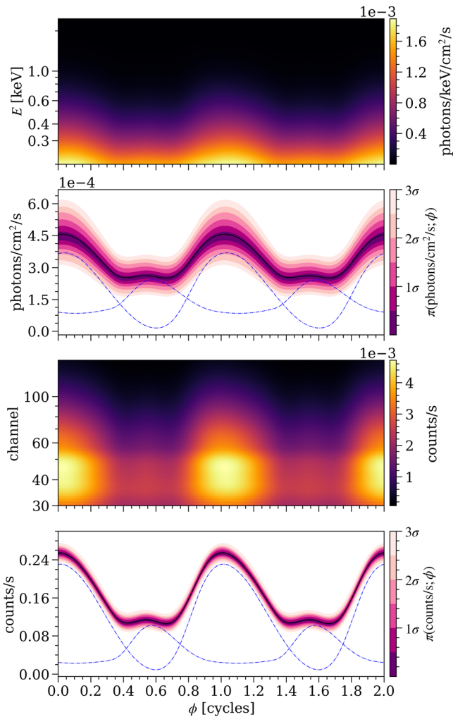
Figure 8. Posterior-expected pulse profiles for the joint NICER and XMM-Newton analysis using the \text{PDT-U} H R_{\text{eq}} \in [10, 14] km model. The top and top-center panels show the signal incident on the telescopes, and the bottom-center and bottom panels show the signal registered by NICER after accounting for the instrument response. The blue-dashed curves show the posterior-expected signals generated by the two hot regions separately and the black-solid curves in combination. The conditional posterior distribution of the incident photon flux and the NICER count rate are also presented (purple contours in the top-center and bottom panels, respectively). See Figure 11 of T. E. Riley et al. (2021) for additional details about the figure elements.
