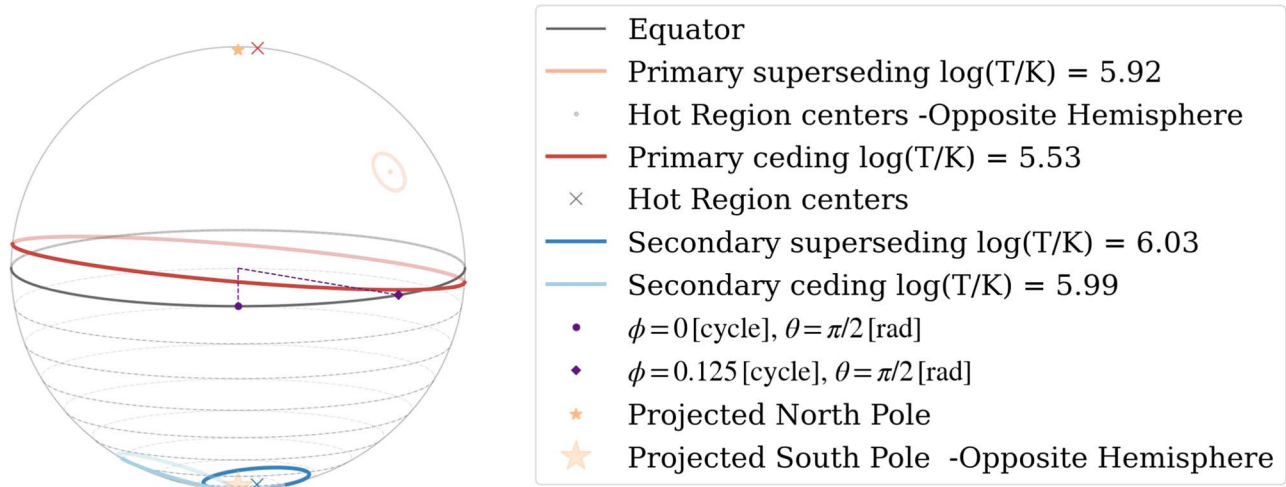
Figure 9. The maximum-likelihood geometry configuration for the joint NICER and XMM-Newton analysis using the PDT-U H R_{\text{eq}} \in [10, 14] km model. The viewing angle represents the Earth’s inclination to the spin axis. The maximum-likelihood geometry is very similar for the PDT-U H R_{\text{eq}} R21 and PDT-U He R_{\text{eq}} R21 models, except that the primary superseding component is located at the equator for the latter.
