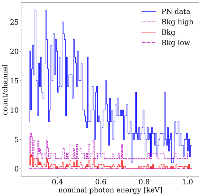
Figure 2. XMM-Newton EPIC-pn camera PSR J1231–1411 count number spectrum as a function of nominal photon energies (blue-stepped curve). The measured rescaled background (red-stepped curve) and the background limits used in the analysis (purple dashed and dotted–dashed stepped curves) are also shown. The choice of the limits is explained in Section 3.4. The complete figure set (3 images), including also the spectra and backgrounds for EPIC-MOS1 and EPIC-MOS2 instruments is available in the online journal (HTML version).
