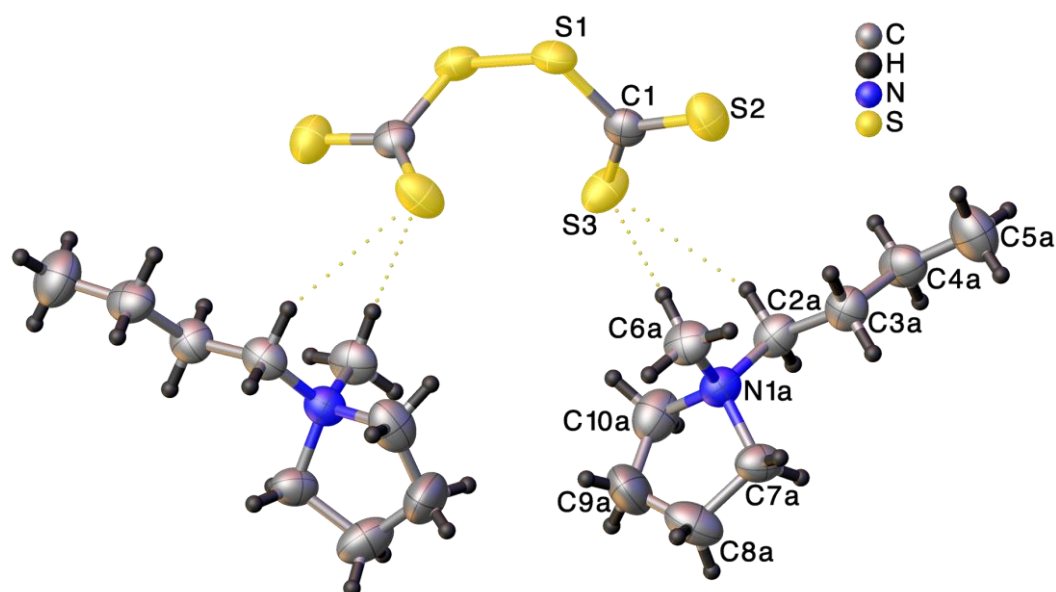
Figure 2. ORTEP (Oak Ridge Thermal Ellipsoid Plot) drawing of the bis(1-butyl-1-methylpyrrolidinium) perthiodicarbonate with thermal ellipsoids at the 50% level. The labeling scheme is shown for the asymmetric unit only. The minority part of the disordered cation is removed for clarity.
