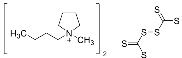
Figure 1. Chemical structure of bis(1-butyl-1-methylpyrrolidinium) perthiodicarbonate 4 .
