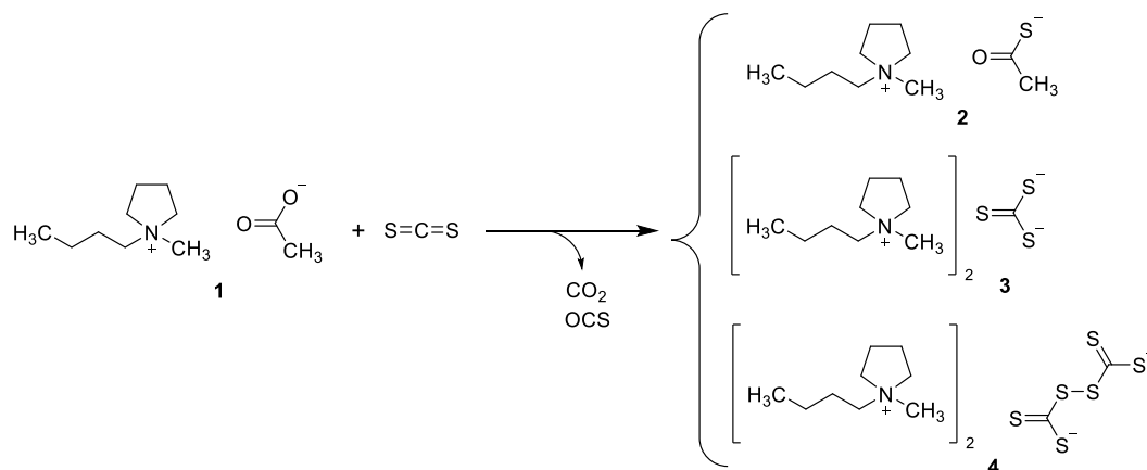
Scheme 1. Synthesis of bis(1-butyl-1-methylpyrrolidinium) perthiodicarbonate 4 .
