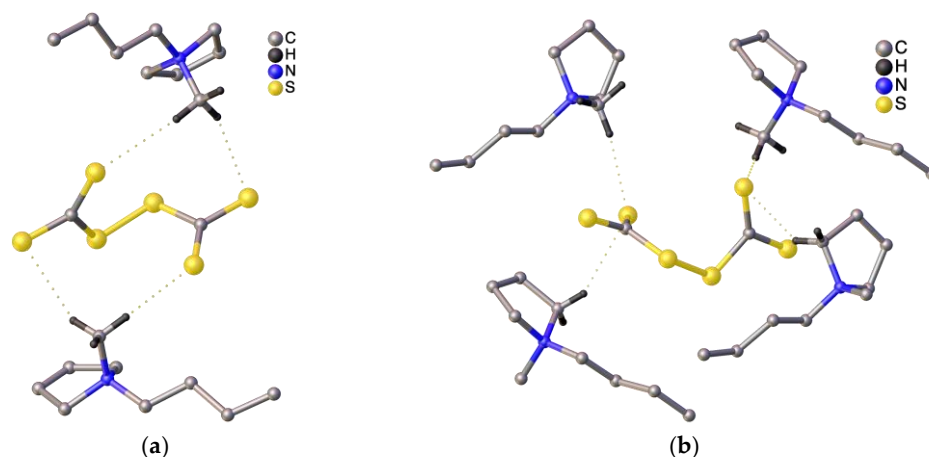
Figure 3. View of the anion–cation interaction showing the (a) double S···H contacts and (b) single S···H contacts.
