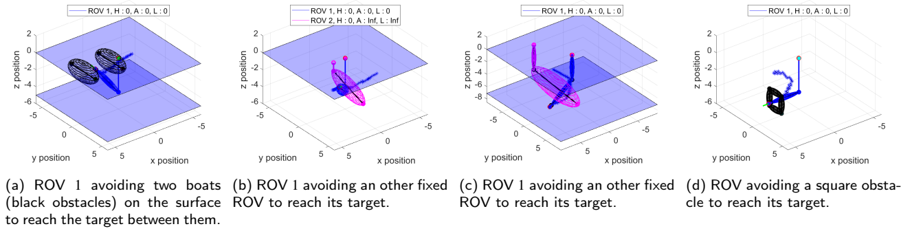
Figure 12: Simulations with one moving ROV and several obstacles. Blue ellipsoid: tether 1. Magenta ellipsoid: tether 2 obstacle. Black ellipsoids: full-obstacles. Blue plane: sea surface.
