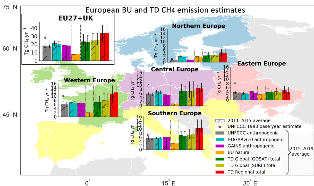
Figure 1. Five-year means (2011–2015, hashed bars, and 2015–2019, full bars) in total CH 4 emission estimates (excluding LULUCF) for the EU27 + UK and five European regions (north, west, central, south and east non-EU). The eastern European region does not include European Russia. Northern Europe includes Norway. Central Europe includes Switzerland. The data come from UNFCCC NGHGI (2021) submissions (gray), which are plotted with respective base year 1990 (black star) estimates, two inventories (GAINS and EDGARv6.0), natural unmanaged emissions (sum of peatland, geological, inland waters (RECCAP2) and GFEDv4.1 biomass burning emissions) and three inversion estimates: one regional European inversion (excluding InGOS unavailable for 2013–2015) and GOSAT and SURF ensemble estimates from global inverse models. The relative error on the UNFCCC value represents the UNFCCC NGHGI (2021) reported uncertainties computed with the error propagation method (95 % confidence interval) and gap-filled to provide respective estimates for each year. Uncertainty for EDGARv6.0 was calculated for 2015 based on the 95 % confidence interval of a lognormal distribution (Solazzo et al., 2021).
