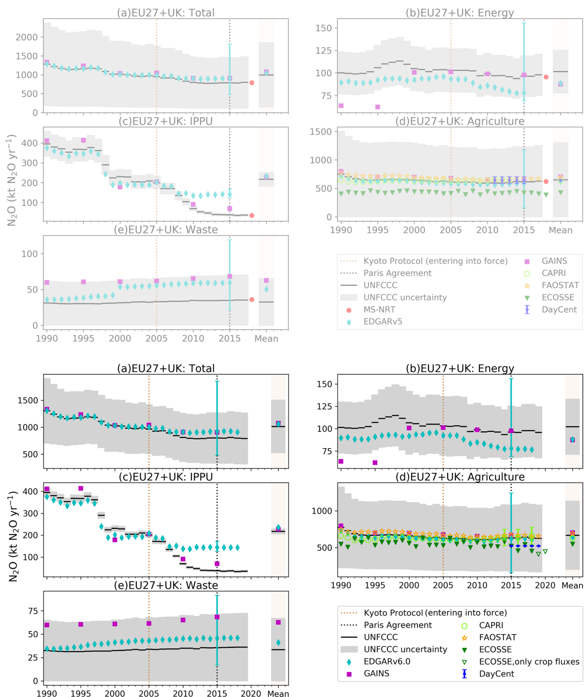
Figure 12. (a) Total annual anthropogenic N 2 O emissions (excluding LULUCF) for the EU27 + UK over time. The top plot presents previous data synthesized in Petrescu et al. (2021), while the bottom plot depicts data synthesized by the current study: (a) EU27 + UK and total sectoral emissions from (b) energy, (c) IPPU, (d) agriculture, and (e) waste from UNFCCC NGHGI (2021) submissions compared to global BU inventories for agriculture (CAPRI, ECOSSE, FAOSTAT, DayCent) and all sectors excluding LULUCF (EDGARv6.0, GAINS). CAPRI reports one value for Belgium and Luxembourg. The relative error on the UNFCCC value represents the UNFCCC NGHGI (2021) member-state-reported uncertainties computed with the error propagation method (95 % confidence interval) that were gap-filled and provided for every year. The uncertainty for EDGARv6.0 is the same as that of v5.0 and calculated for 2015 as min/max values for the total and each sector (Solazzo et al., 2021) and represents the 95 % confidence interval of a lognormal distribution. CAPRI reports uncertainties for the last 3 years as follows: 2014 and 2016 (17.6 %) and 2018 (17.8 %). The mean column represents the common overlapping period of 1990–2018 between datasets. The last years of the time series of the respective datasets are 2019 (UNFCCC and FAOSTAT), 2018 (EDGARv6.0, CAPRI), 2015 (GAINS every 5 years), 2015–2019 (DayCent) and 2020 ECOSSE, with the last 2 years reporting only crop emissions.
