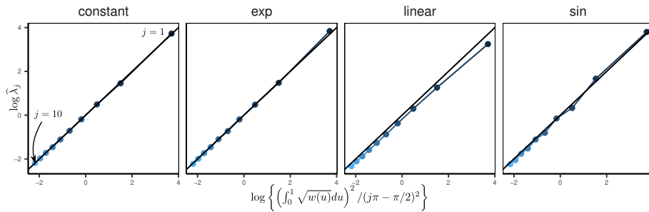
FIG 2. Average eigenvalues ( \log -scale) for Poisson Processes over 50 replicated. Each dot corresponds to a value of j \in \{1, \dots, 10\} . The empirical average is plotted vs the expected theoretical asymptotic regime of eigenvalues in (\int_0^1 \sqrt{w(u)} du)^2 / (j\pi - \pi/2)^2 , as expected from Theorem 4.4. Note that Theorem 4.4 provides a (j\pi)^{-2} regime. The black line corresponds to the first bisector, so that the points align if the empirical convergence matches the theoretical regime.
