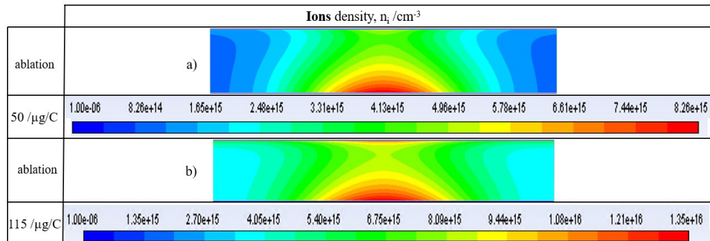
Figure 5. Fields of the ion density for an ablation rate of a) 50 \mu\text{g}/\text{C} and b) 115 \mu\text{g}/\text{C} , I = 15 \text{ kA} , B_{AMF} = 75 \text{ mT} .
