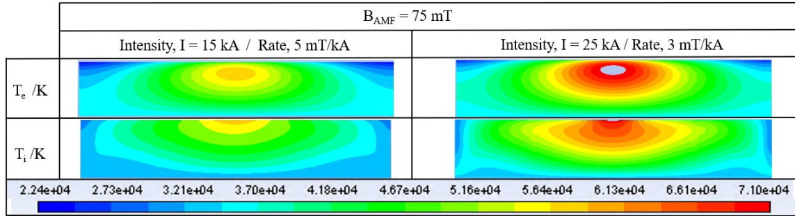
Figure 7. Fields of the electron and ion temperature for several values of current intensity, I = 15 kA and I = 25 kA, B_{AMF} = 75 mT, the ablation rate is 50 \mu\text{g/C} .
