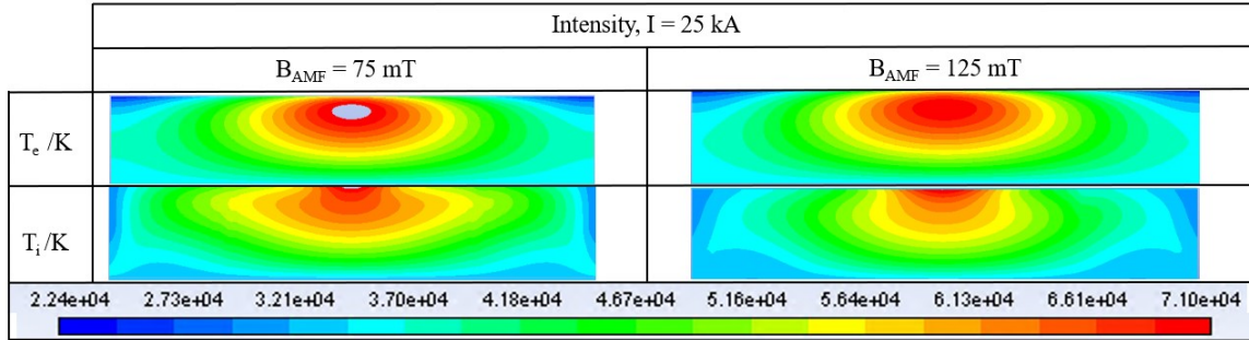
Figure 6. Fields of the electron and ion temperature for several values of the axial magnetic field, B_{AMF} = 75 mT and B_{AMF} = 125 mT, I = 25 kA, the ablation rate is 50 \mu\text{g/C} .
