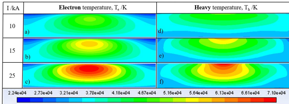
Figure 8. Fields of electron and ion temperature for several values of current intensity I = 10 kA and B_{AMF} = 50 mT, I = 15 kA and B_{AMF} = 75 mT, I = 25 kA and B_{AMF} = 125 mT, ablation rate is 50 \mu\text{g/C} , rate is 5 mT/kA.
