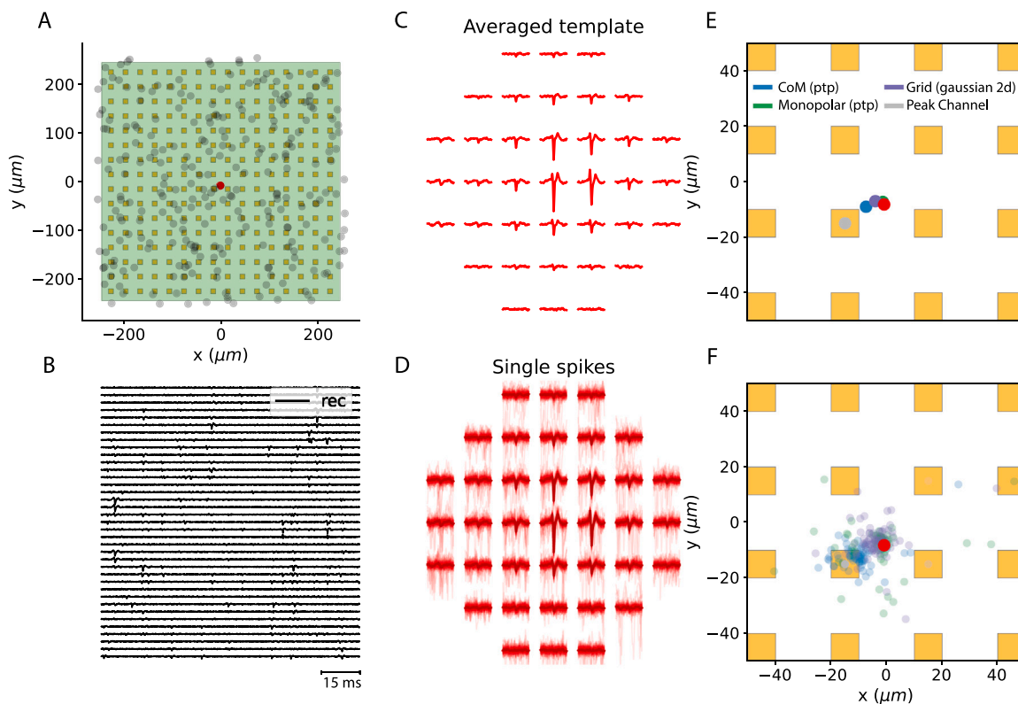
Fig. 1. Illustration of the generation of artificial recordings. A The layout of a 256-channel HD-MEA with 30\ \mu\text{m} spacing between each electrode is displayed, and the black dots correspond to the positions of (some of) the artificial neurons. The red dot highlight the particular case of the neuron whose waveforms are shown in panels C , D . B 100 ms of extracellular recordings, shown only for a few channels. C The template of the neuron highlighted in red in panel A (averaged over many spikes). D 100 waveforms taken from single spikes of the same neuron (as in C ), superimposed. E Localization, with several localization algorithms (see Methods), performed on the averaged template. Red dot illustrates the real position of the generated template. F Same as E , but when localizing individual spikes.
