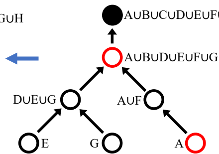
(e) Max-tree
