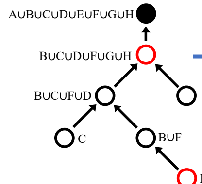
(f) Min-tree
