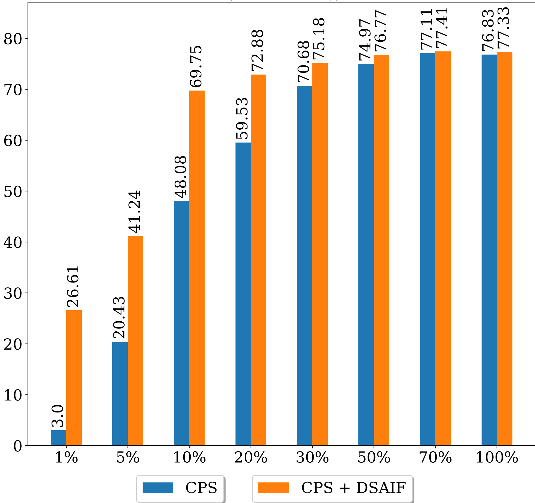
Jaccard Index (%) (PROMISE12))
