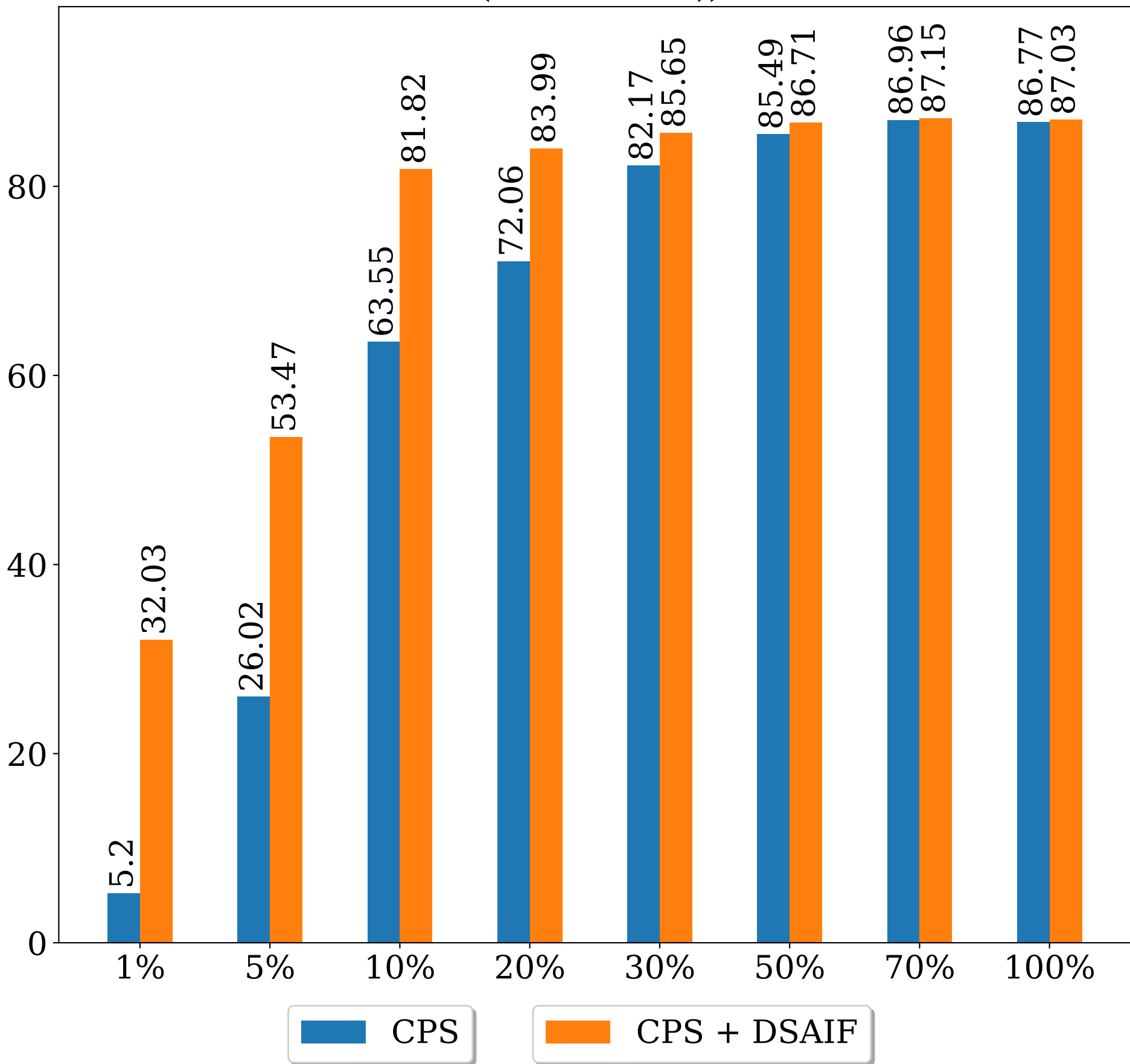
Dice Coefficient (%) (PROMISE12))
