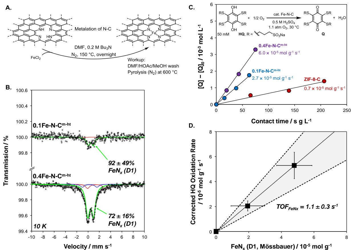
Figure 2. (A) Preparation of atomically dispersed Fe-N-C catalysts via solution-phase metalation and heat treatment. Planar tetrapyrrolic sites are shown as an example. (B) 57 Fe Mössbauer spectra (10 K) of 0.1Fe-N-C m-ht (top) and 0.4Fe-N-C m-ht (bottom). Data (open points) are fit with a sum (black line) of components assigned to Fe III N x (D1, green), Fe II N x (D2, blue), FeCl 2 ·4H 2 O (D3, red), and FeO x clusters (S1, gray). (C) Concentration of quinone formed as a function of contact time on 0.4Fe-N-C m-ht (purple) and 0.1Fe-N-C m-ht (blue). The Fe-free analog (ZIF-8-C) is shown in red. Conditions: 30 °C, 1.1 bar O 2 , 0.5 M H 2 SO 4 , [HQ] 0 = 50 mM, [Q] 0 = 1 mM. Lines reflect regressed fits constrained through the origin. (D) Correlation of the Fe-catalyzed HQ
