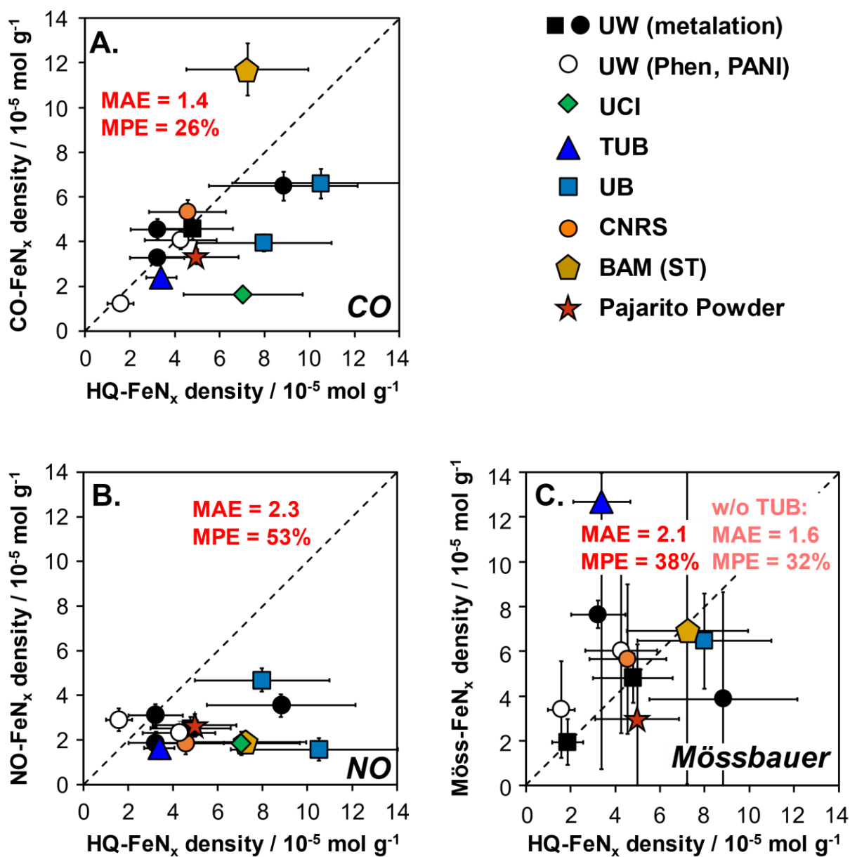
Figure 5. Parity plots comparing spectroscopic and probe-molecule \text{FeN}_x site quantification methods with the kinetic method. The dashed lines indicate equality between the two values. All x-axes reflect kinetically quantified \text{FeN}_x site densities derived from hydroquinone oxidation rates and the intrinsic TOF of \text{FeN}_x sites ( 1.1 \pm 0.3 \text{ s}^{-1} ). The y-axes reflect (A) CO pulse chemisorption, and (B) stripping of NO derived from \text{NO}_2^- , and (C) Mössbauer spectroscopy. The mean absolute error (MAE) and mean percentage error (MPE) associated with each correlation are calculated according to eq S9 and S10 in the Supporting Information and shown in the plot area. The two x\text{Fe-N-C}^{\text{m-ht}} materials (black squares) are omitted from the MAE and MPE values in (C) because they were used to estimate \text{TOF}_{\text{FeN}_x} (Figure 2D) and so N_{\text{FeN}_x, \text{HQ}} and N_{\text{FeN}_x, \text{Möss}} are not independently determined. The MAE and MPE values in (C) without the outlier 5.7Fe-N-C-TUB are reported in pale red text.
