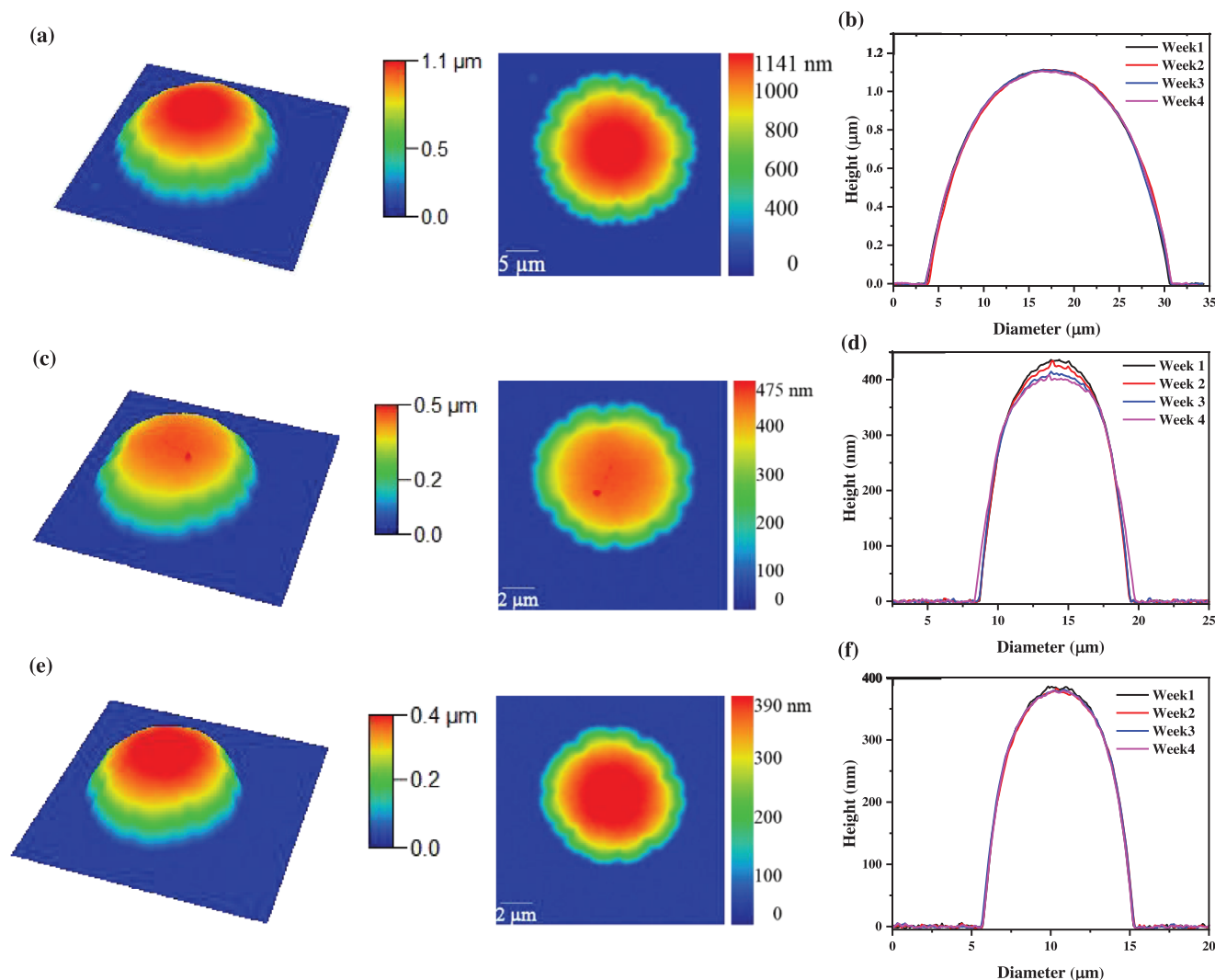
Figure 5. 3D and 2D AFM images of h-BN bubbles with a) d = 27 \mu\text{m} and h = 1.1 \mu\text{m} , c) d = 10.9 \mu\text{m} and h = 434 \text{ nm} , and e) d = 9.8 \mu\text{m} and h = 376 \text{ nm} . b,d,f) AFM cross-sectional profile of h-BN bubbles shown in (a,c,e), respectively.
