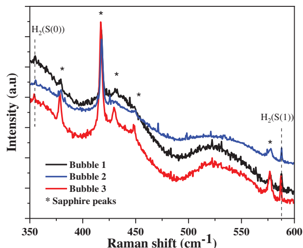
Figure 1. Raman spectroscopy of different h-BN bubbles, showing the vibrational modes S(0) and S(1) of H 2 molecule located at 354 and 587 \text{cm}^{-1} , respectively.
