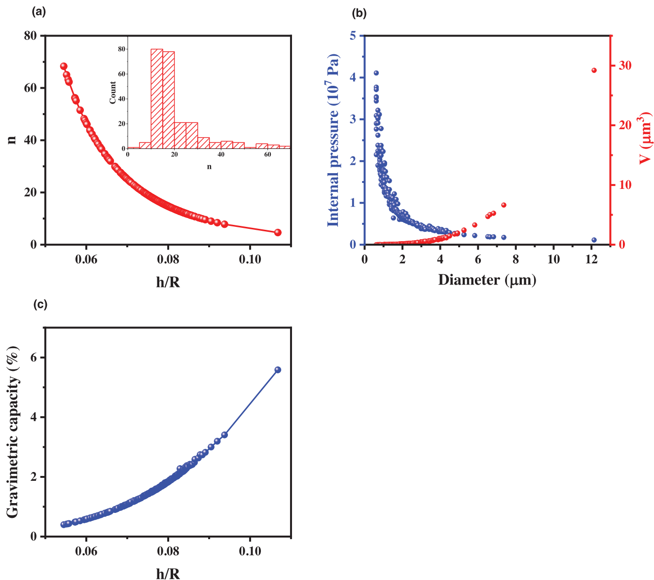
Figure 8. a) The number of atomic layers on the top of h-BN bubbles as a function of aspect ratio h/R . b) Variation of internal pressure and volume of h-BN bubbles versus the bubble diameter. c) Hydrogen storage capacity C of h-BN bubble as a function of aspect ratio h/R .
