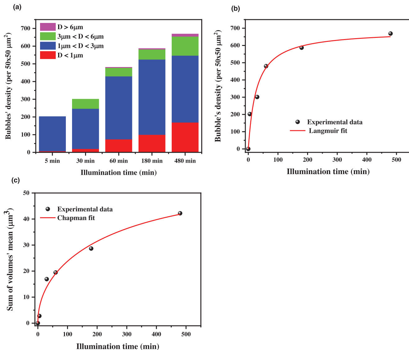
Figure 3. Influence of UV laser illumination time on h-BN bubble size. a) Histogram of h-BN bubble density. b) Variation of h-BN bubble density as a function of illumination time. c) Total mean volume for each illumination duration as a function of illumination time.
