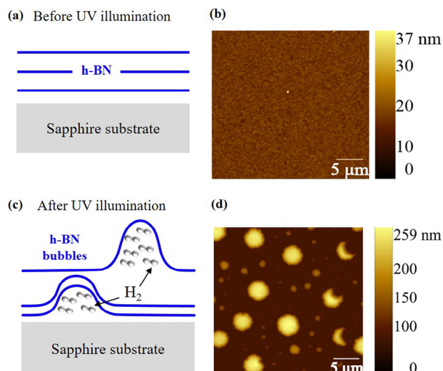
Figure 2. a) Schematic illustration and b) AFM image of h-BN on sapphire substrate. c) Schematic illustration and d) AFM image of h-BN on sapphire substrate irradiated by UV laser.
