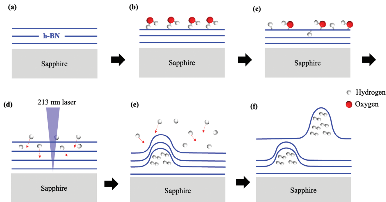
Figure 6. a) h-BN film grown using MOCVD on sapphire substrate. b) Adsorption of water molecule on h-BN nanosheets. c) Dissociation of water molecules on vacancy sites in h-BN into N–H and OH–B bonds. d) Sample exposure to 213 nm UV laser light. e) Diffusion and recombination of hydrogen protons upon UV exposure. f) Formation and confinement of hydrogen gas molecules inside h-BN bubbles.
