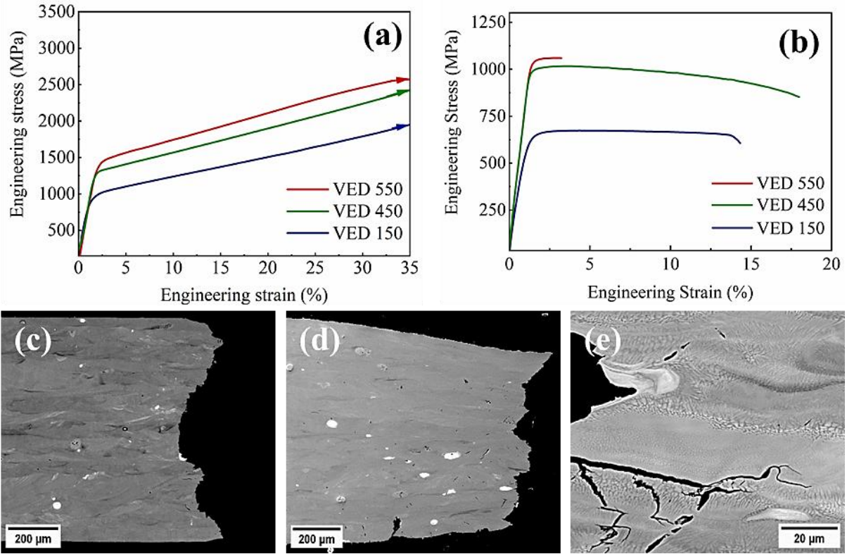
155 FIG. 3. (a) Typical stress-strain compression test plots of the synthesized alloys along the Z axis/OXY 156 plane (building direction), (b) tensile test plots along the OYZ plane, (c, d) failure profiles of the 157 tensile tested 550 and 450 J.mm -3 specimens, respectively and (e) crack propagation along the HAGBs 158 in the tensile tested 450 J.mm -3 specimen. 159
