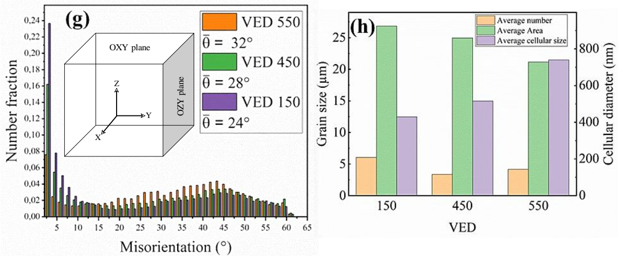
120 FIG. 2. Microstructure quantification details. (a-c) IP EBSD images superimposed to the grain 121 boundaries map of the VED = 150, 450 and 550 J \cdot mm^{-3} specimens, respectively, (d-f) SEM images of 122 the cellular substructure of each specimen and (g, h) distribution of the misorientation across the grain 123 boundaries, frequency of grain, and cellular size as a function of the applied VED (Z axis in Fig (g) 124 indicates the laser beam direction). 125
