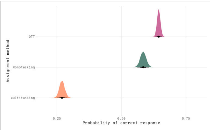
Figure 5. Posterior probability distributions (with mean and 95% CI) of the probability estimates that responses will match each one the three assignment methods in the task assignment phase.
