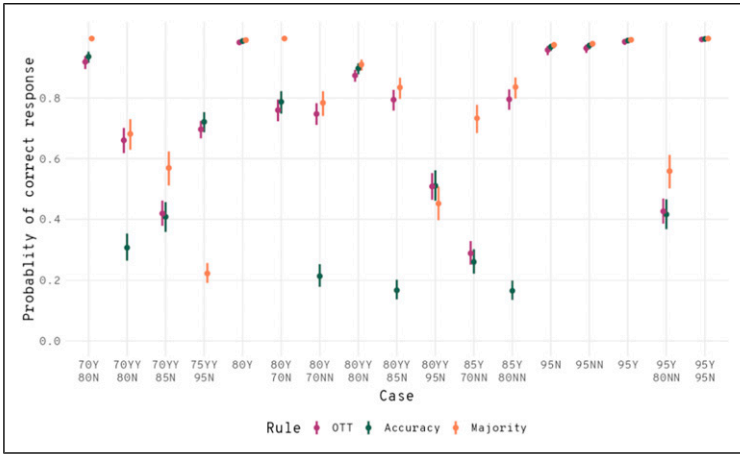
Figure 10. Mean (with 95% CI) estimates per case of the probability that participants' responses correspond to each one of the decision rules in the aggregation phase.
