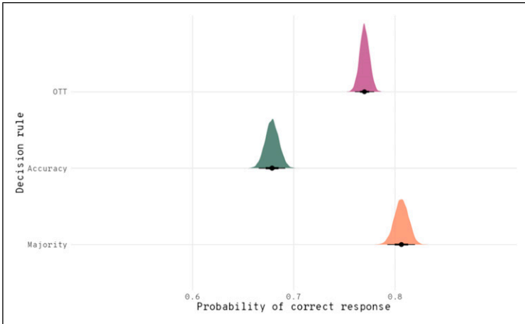
Figure 9. Posterior probability distributions (with mean and 95% CI) of the probability estimates that responses will follow each decision rule in the aggregation phase.
