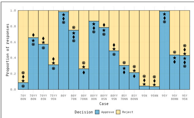
Figure 8. Proportion of participants' aggregation decisions for each case. (★) indicates response(s) predicted by the OTT rule, (◆) those predicted by the accuracy rule and (⊗) those predicted by the majority rule.
