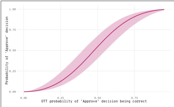
Figure 11. Conditional effects plot (with 95% compatibility interval) for the relationship between the probability of an 'Approve' decision being correct according to the OTT rule and the probability that a participant will choose the 'Approve' response.
