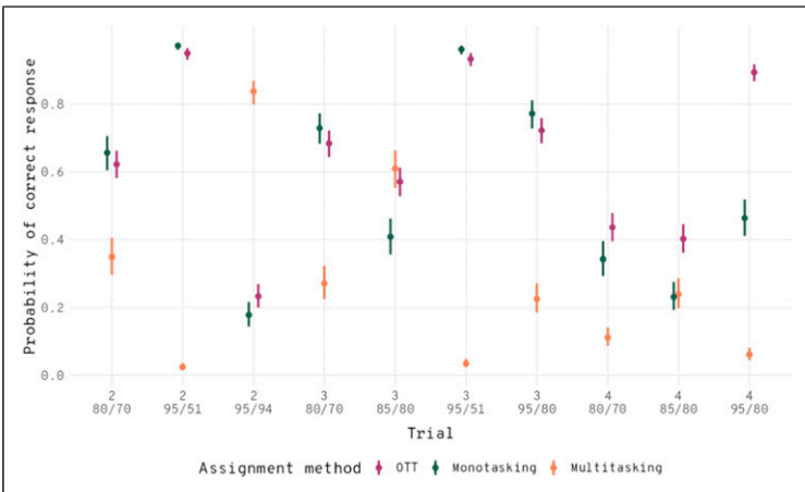
Figure 6. Mean (with 95% CI) estimates per trial of the probability that participants' responses correspond to each one of the decision rules in the task assignment phase.
