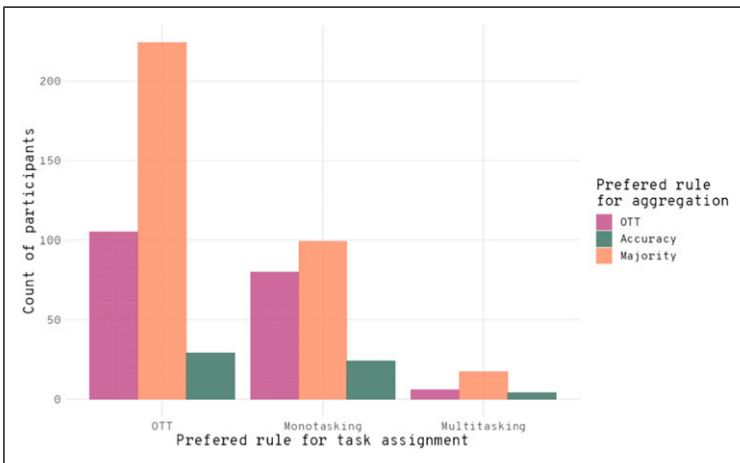
Figure 12. Counts of participants according to whether they were estimated, by Models 1 and 4, as favouring one of the three competing decision rules for the task assignment and aggregation parts.
