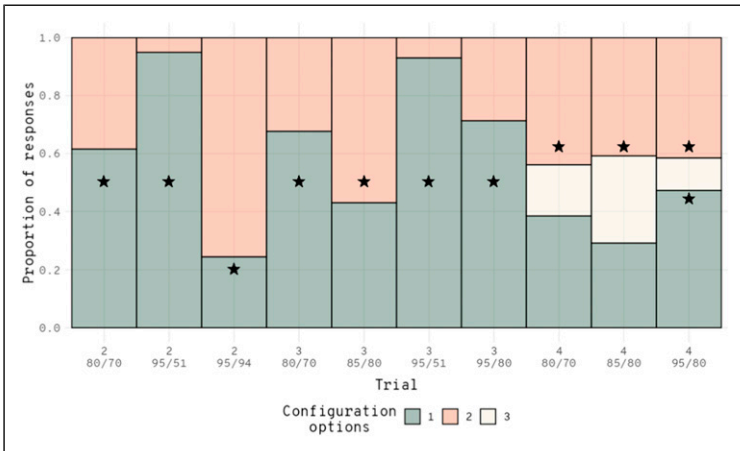
Figure 4. Proportion of participants' task assignment decisions for each trial. (★) indicates the response(s) predicted by the OTT assignment method. The monotasking assignment method predicts that option 1 will be chosen for all cases and the multitasking assignment method predicts that option 2, or 3 when available, will be chosen for all cases.
