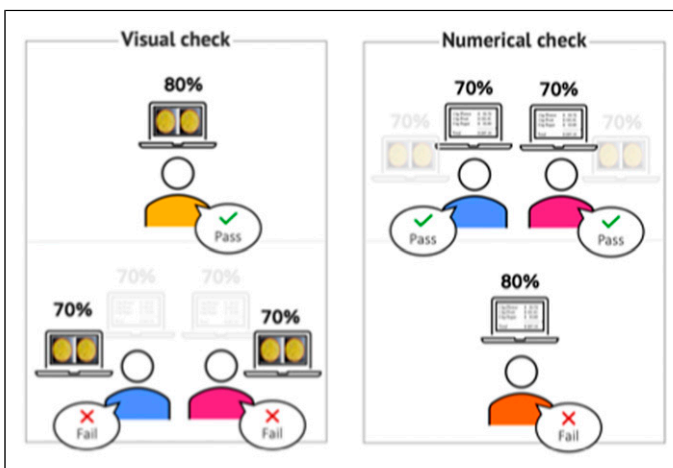
Figure 3. Aggregation trial for a team of size 4, with q = 0.80 and p = 0.70 .
