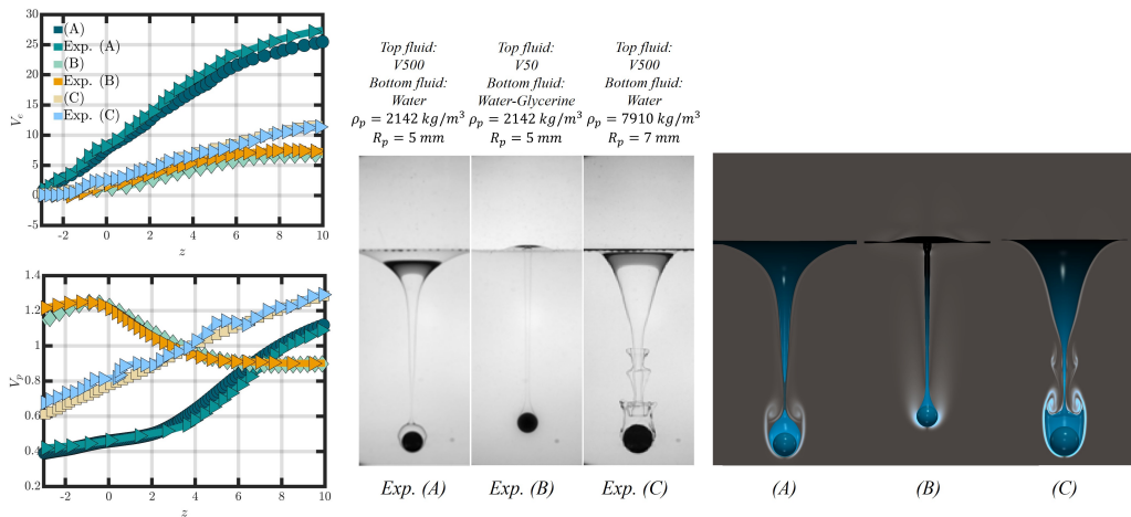
Figure 16: This figure showcases the experimental results of Pierson & Magnaudet (2018 a,b ) for a spherical particle crossing an immiscible interface under different configurations. The plots showcase the performance of this numerical method compared to the experimental results in estimating the entrained fluid volume V_e and the particle velocity. Qualitative results from the simulations are also provided.
