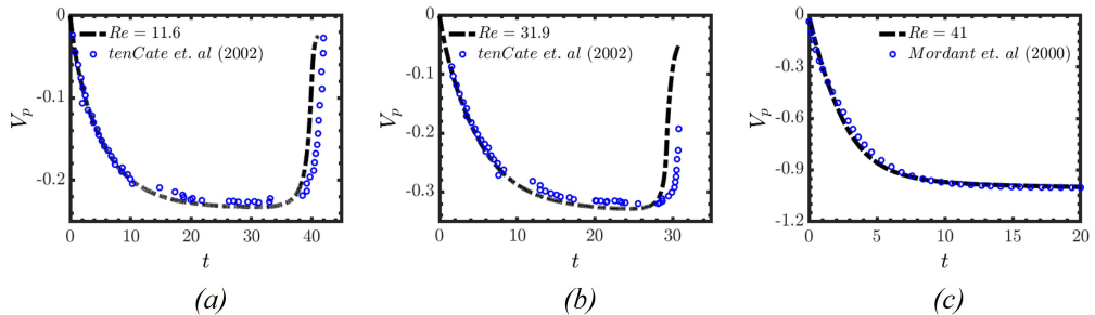
Figure 3: Validation of the numerical technique: comparison of the temporal evolution of the particle settling velocity obtained from our predictions and published experimental data; (a) and (b), and (c) show results for Re = 11.6 and 31.9 (Ten Cate et al. 2002), and Re = 41 (Mordant & Pinton 2000), respectively.
