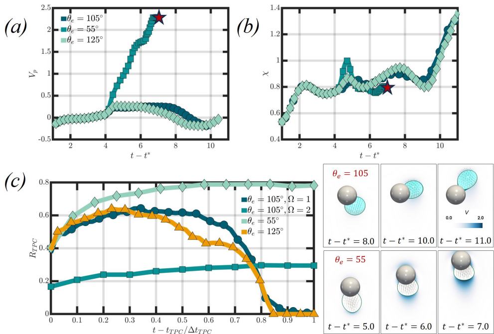
Figure 11: This figure showcases the dynamics of the interaction after the formation of the contact line, when Ga = 10 , Bo = 0.5 , and \zeta_p = 1 . In panel (a), the particle’s vertical velocity is presented for different particle wettability parameters, which correspond to a base case with \theta_e = 105^\circ , and two additional cases with \theta_e = 55 , and \theta_e = 125 . The figures on the right-hand side correspond to t - t^* from 8 to 11 for the base case and t - t^* from 5 to 7 when \theta_e = 55^\circ . Panel (b) showcases the aspect ratio \chi for the three different cases, and the pentagram indicates reaching the top boundary. Lastly, panel (c) showcases the temporal evolution of radius of the contact line R_{TPC} when varying \theta_e and \Omega . Note that the x -axis is scaled with the contact line time t_{TPC} .
