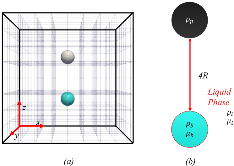
Figure 1: (a) The three-dimensional Cartesian cubic domain with a size of 16R \times 16R \times 16R , showing the subdomain decomposition and the initial problem setup; (b) the initial separation distance between the particle and the bubble is shown.
