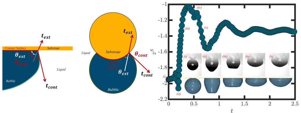
Figure 15: The left hand side of the figure provides an illustration of the contact line numerical methodology between a bubble and a solid wall or solid particle. The plot showcases the temporal evolution of the south pole of the bubble as it adheres to a solid wall with negligible inertia. The contact angle for this case was \theta_A = 102 , \theta_R = 99 . A qualitative comparison with the experimental results of Basarova et al. (2018) is provided at different time steps.
