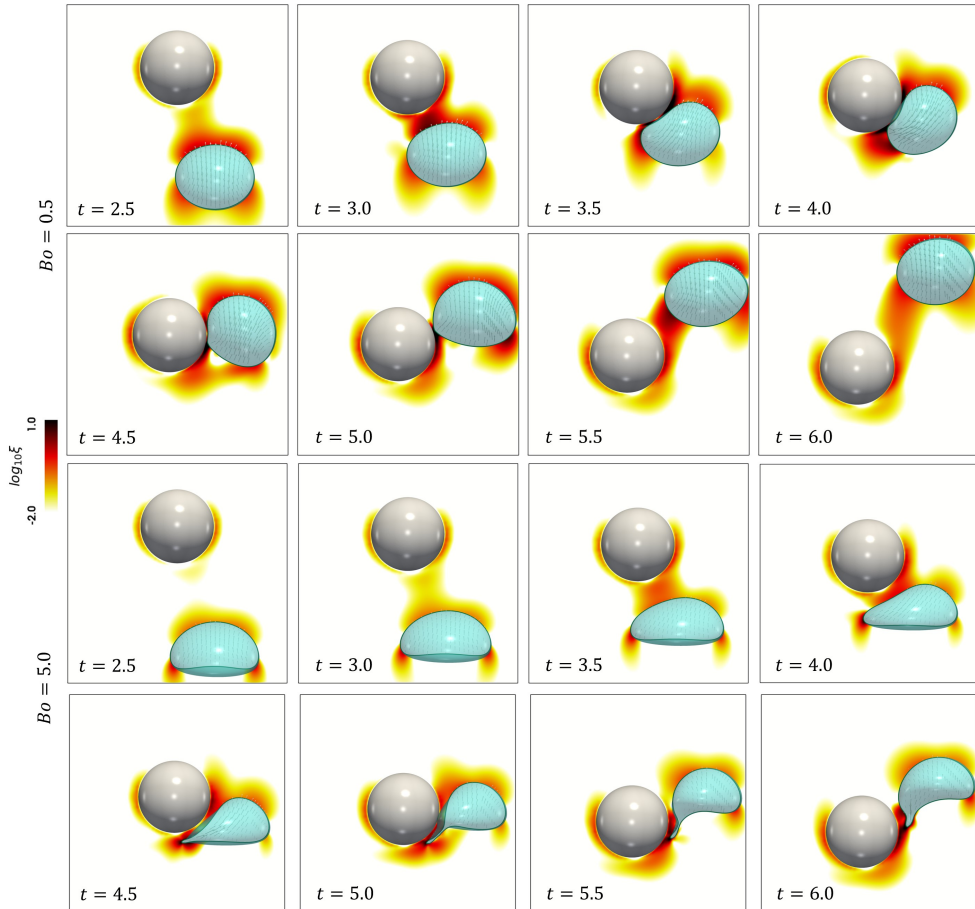
Figure 12: Spatio-temporal evolution of off-centre bubble-particle interaction dynamics with Ar = 10 , Ga = 10 , and an initial bubble location offset of \delta = 1 . The results shown in the top and bottom two rows were generated with Bo = 0.5 and Bo = 5 , respectively. The contours are of the logarithm of the viscous dissipation function \log_{10} \xi in the fluid. The bubble is shown with glyphs of the velocity to illustrate the relative motion of the bubble at different time-steps. The snapshots are shown between t = 2.5 and t = 6 in time-increments of \delta t = 0.5 .
