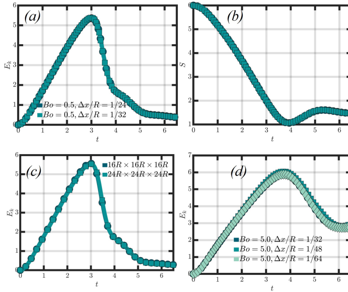
Figure 14: The top two panels (a) and (b) show the total kinetic energy of the system and the distance between the particle south pole and the bubble south pole ( S ), at two different resolutions for Ga = 10 , Bo = 0.5 , and \zeta_p = 1 , respectively. Panel (c) shows the temporal evolution of the total kinetic energy when increasing the domain size for the same case. It can be seen that increasing the domain size leads to no difference in the results. Panel (d) shows the total kinetic energy for different mesh sizes for Ga = 10 , Bo = 5.0 , and \zeta = 1 , up to a resolution of \Delta x/R = 1/64 . The results show that the domain size and mesh resolution utilised in this work is sufficient to capture the dynamics of the interaction between the bubble and the particle.
