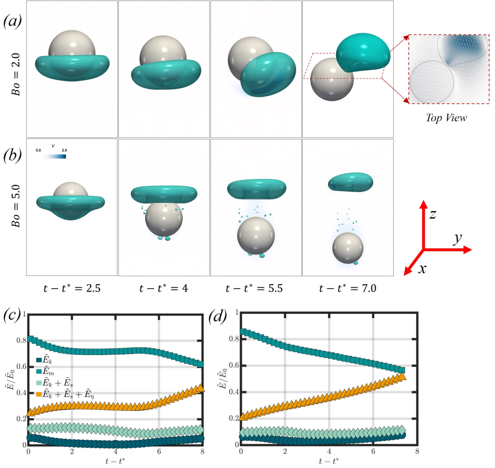
Figure 7: The spatio-temporal evolution of the bubble-particle interaction dynamics is shown in (a) for Ga = 10 , Bo = 2 and \zeta_p = 1 , where the contours depict the velocity magnitude. Panel (b) shows the spatio-temporal evolution of the interaction dynamics when Ga = 10 , Bo = 5 and \zeta_p = 1 . The timesteps presented are relative to t^* , such that t - t^* varies from 2.5 to 7.0. When Bo = 2 and t - t^* = 7 , a top view of the interaction between the bubble and the particle is presented to showcase that no contact is found between them. In panels (c) and (d), the normalised energy budget \tilde{E}/\tilde{E}_0 is presented for Bo = 2 and Bo = 5 , respectively, where \tilde{E}_0 = E_{p_0}^{particle} + E_{s_0} .
