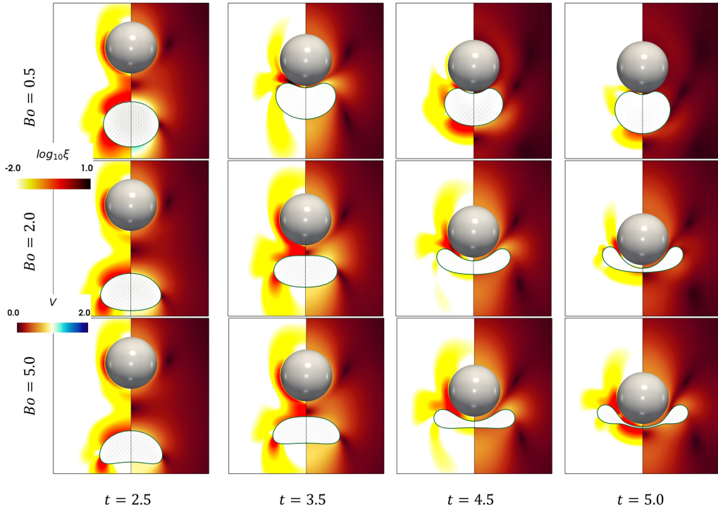
Figure 6: Spatio-temporal evolution of the bubble-particle interaction dynamics shown for the same parameters used to generate Figure 4; the rows are associated with Bo = 0.5 , Bo = 2.0 , and Bo = 5 , from top to bottom. The contours on the left part of the figures in the panels show the logarithm of the viscous dissipation function \log_{10} \xi in the fluid, and the contours on the right show the velocity magnitude in the fluid V . The bubble is shown with glyphs of the velocity to illustrate the relative motion of the bubble at different time-steps.
