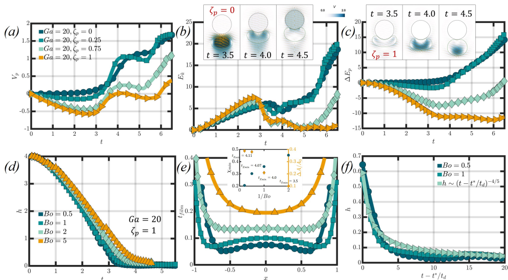
Figure 10: In panels (a), (b) and (c), the particle settling velocity, total kinetic energy, and the change in particle potential energy are presented, respectively. These results correspond to when Ga = 20 , Bo = 0.5 and varying \zeta_p . Temporal evolution of the minimum gap thickness h_m(t) is shown in (d) for \zeta_p = 1 , Ga = 20 , and Bo = [0.5 - 5] ; an enlarged view of the plot in (d) is shown in panel (e), for Bo = 0.5 and Bo = 1 as at these Bo numbers, the bubble did not rupture. A scaling for the film drainage is provided such that h \sim (t - t^*)/t_d^{-4/5} . Panel (e) showcases the film thickness profile at t_{\chi_{min}} when varying Bo and maintaining Ga = 20 and \zeta_p = 1 .
