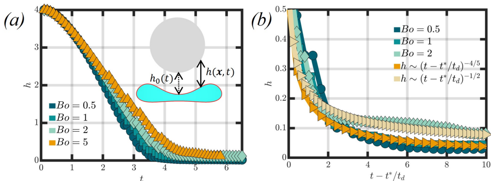
Figure 8: Panels (a) and (b) show the temporal evolution of the minimum gap thickness h(t) for different Bo when Ga=10 and \zeta_p = 1 . Two different scaling are also provided, such that h \sim (t - t^*/t_d)^{-\alpha} where \alpha here is either -4/5 or -1/2 .
