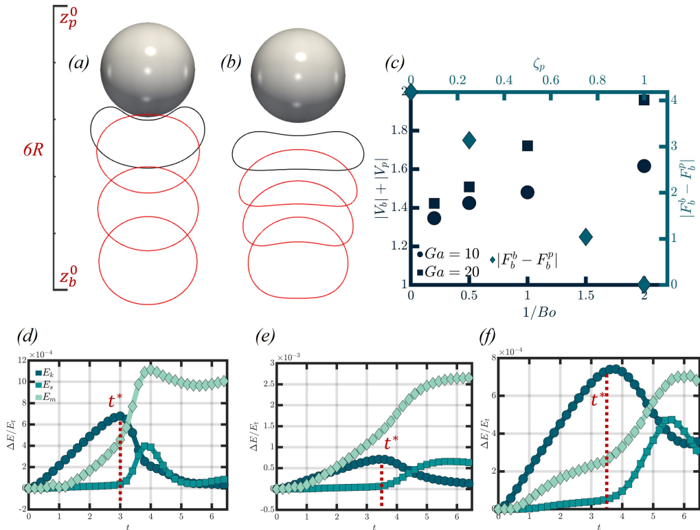
Figure 4: Spatio-temporal evolution of the rising bubble as it approaches the particle is shown in (a) and (b). The snapshots of the bubble contours are shown for t = 1, 2, 3, 4 , and the particle is only shown at t = 4 . In panel (a), a scale indicating the separation distance is provided between the bubble and the particle, indicating the bubble and the particle's initial centre positions at z_b^0 and z_p^0 , respectively. The non-dimensional parameters are (a) Bo = 0.5, Ga = 10, Ar = 10 , (b) Bo = 5, Ga = 10, Ar = 10 ; panels (d), (e) and (f) show the change in energy of the system for three different Bo numbers and maintaining Ga = 10 , and they are Bo = 0.5, Bo = 2.0 , and Bo = 5.0 , respectively. Here, E_m is the mechanical energy of the system, such that \Delta E_m = \Delta E_p + E_k . A new timescale is introduced here, t^* , which corresponds to the time for the reversal of kinetic energy due to the interaction. Panel (c) showcases the relative velocity of the bubble and the particle when varying Bo and Ga at t^* , and also showcases the difference in buoyancy force between the bubble and the particle when varying \zeta_p .
