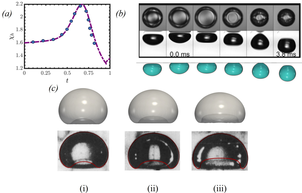
Figure 2: Validation of the numerical technique: Panels (a) and (b) show a comparison of our predictions with the experimental data of Kosior et al. (2014) for a freely-rising bubble interacting with a solid wall; (a) compares the bubble deformation as a ratio of the horizontal over the vertical bubble axis, and (b) depicts the spatio-temporal evolution of the bubble-wall collision; (c) (i)-(iii) compare the results of a rising bubble shape with the experimental results of Bhaga & Weber (1981). The top panel shows the three-dimensional illustrations of the terminal bubble shapes, and the bottom panel illustrates a slice of the interface superposed on the experimental results of Bhaga & Weber (1981). The parameter values are (Ga, Bo) = (2.316, 29) , (3.094, 29) , and (4.935, 29) for panels (i), (ii), and (iii), respectively.
