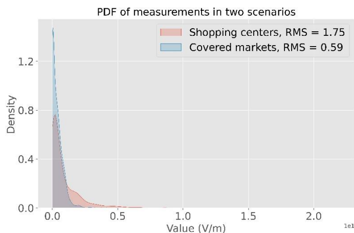
Figure 2: Probability Density Function (PDF) of measurements in two main scenarios.
