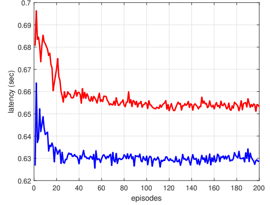
Fig. 4: Average latency and best latency per episode.
