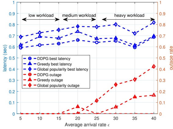
Fig. 6: Performance comparison of three algorithms.
