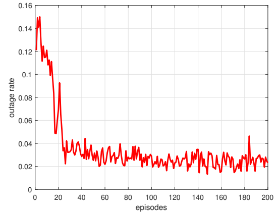
Fig. 5: Average outage rate per episode.
