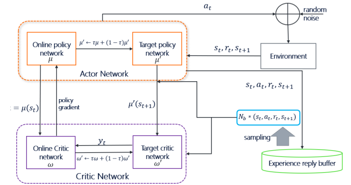
Fig. 2: The structure of DDPG algorithm.
