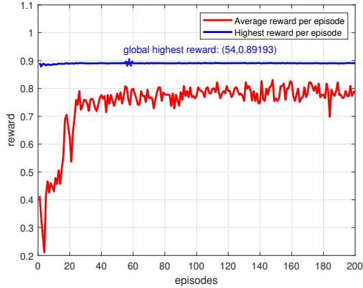
Fig. 3: Average reward and highest reward per episode.
