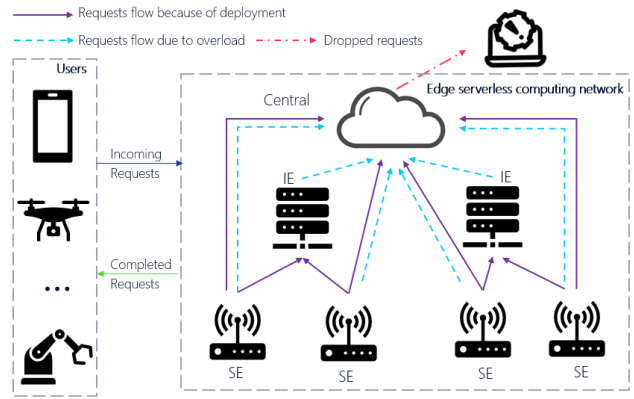
Fig. 1: An example of the service model.
