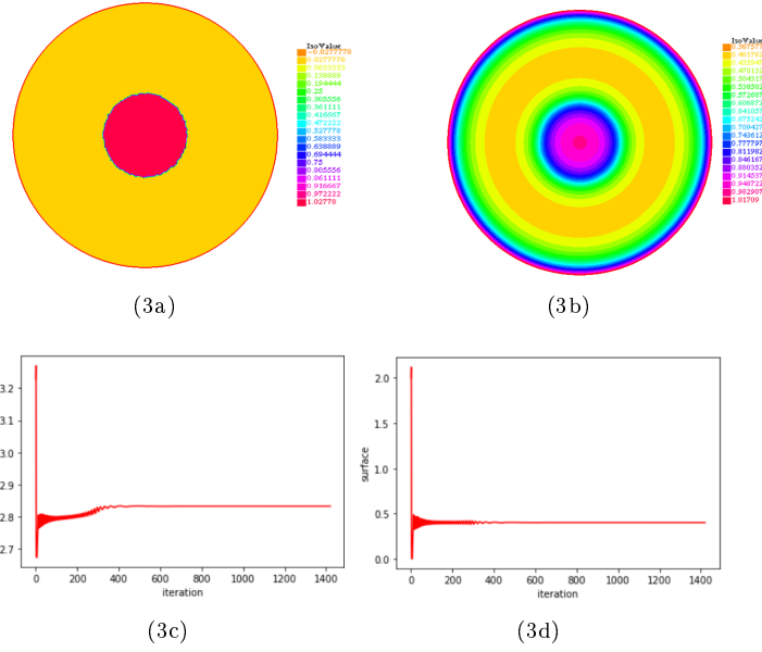
Figure 3: (3a) The optimal control on the circular domain \Omega_3 . (3b) The protection for the optimal control at the final time T . The values of the cost functional (3c) and the surface of the intervention zone (3d) with respect to the iterations.
