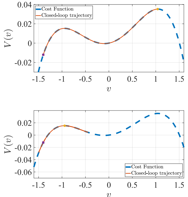
Figure 2: Graph of the cost function (36) and evolution of V(Ex) of two different trajectories of the closed-loop system. The purple square depicts the initial conditions and the yellow circle the converging equilibrium point. The top figure has an initial condition x = [0 \ -1.2 \ 0 \ 0 \ 0 \ 0]^T , while the bottom figure at x = [-10 \ -1.2 \ -0.8 \ 174.13 \ 3.7 \ 0.97]^T .
