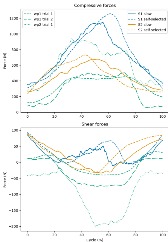
Figure 1. Compressive and shear forces for all subjects and all trials – Comparison between this study (S1, S2) and Orthoload (wp1, wp2). credit: Hinnekens
