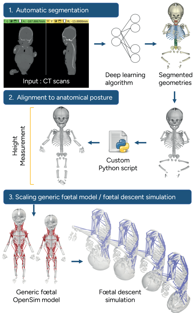
Figure 1. Modelling workflow.
