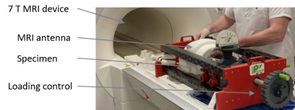
Figure 1. Specific loading device.
