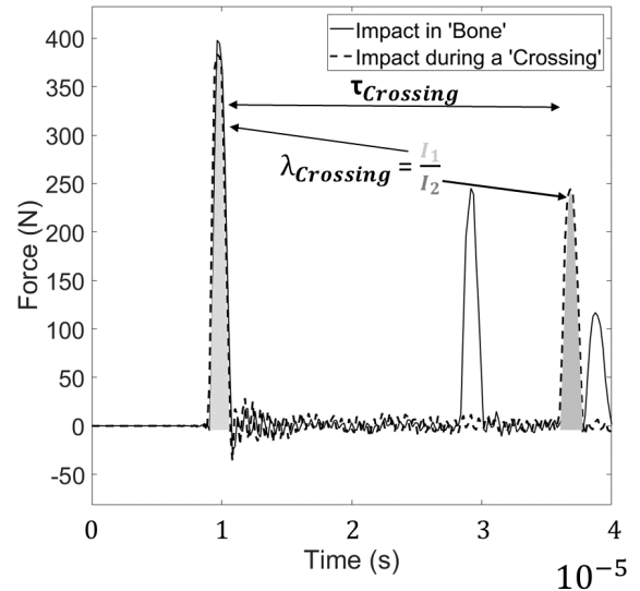
Figure 1. Example of a part of two signals s(t) , variation of the force as a function of time, for an impact in 'Bone' and an impact during a 'Crossing'
